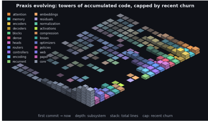
Figure 4: Praxis’s git history as an isometric terrain over the last 2285 commits. Each cell is one subsystem in one time window: a stack of base blocks for its accumulated size (total lines, recency-weighted) topped by a vivid cap for that window’s line churn - the standing codebase carrying the recent activity. Both are weighted by recency (the kernel the model applies to a sequence, turned on the repository): recent windows stack tall with bright caps while history thins toward the always-present prior - the low valley we roll into. Color fades from each subsystem’s hue toward a neutral prior into the past, banded in phased strata over a non-linear timescale. It is the bias/variance geometry read along the frequency axis (see the project notes): loud recent corrections over the quiet, ever-present base. By recency-weighted churn the current center of gravity is core, web, encoders. The framework charts the hand that builds it.
