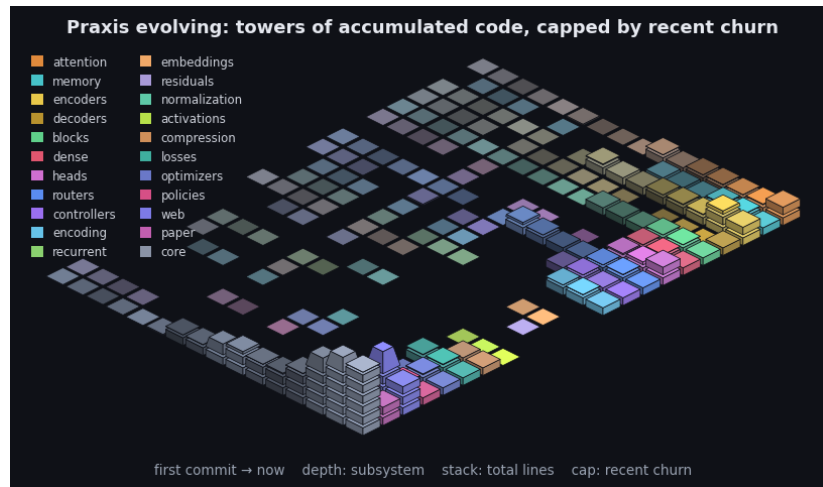
Figure 10: Praxis’s git history as an isometric terrain over the last 2399 commits. Each cell is one subsystem in one time window: a stack of base blocks for its accumulated size (total lines, recency-weighted) topped by a vivid cap for that window’s line churn - the standing codebase carrying the recent activity. Both are weighted by recency (the kernel the model applies to a sequence, turned on the repository): recent windows stack tall with bright caps while history thins toward the always-present prior - the low valley we roll into. Color fades from each subsystem’s hue toward a neutral prior into the past, banded in phased strata over a non-linear timescale. It is the bias/variance geometry read along the frequency axis (see the project notes): loud recent corrections over the quiet, ever-present base. By recency-weighted churn the current center of gravity is core, web, paper. The framework charts the hand that builds it.
