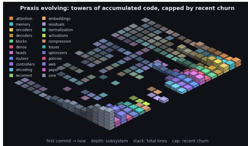
Figure 12: Praxis’s git history as an isometric terrain over the last 2438 commits. Each cell is one subsystem in one time window: a stack of base blocks for its accumulated size (total lines, recency-weighted) topped by a vivid cap for that window’s line churn - the standing codebase carrying the recent activity. Both are weighted by recency (the kernel the model applies to a sequence, turned on the repository): recent windows stack tall with bright caps while history thins toward the always-present prior - the low valley we roll into. Color fades from each subsystem’s hue toward a neutral prior into the past, banded in phased strata over a non-linear timescale. It is the bias/variance geometry read along the frequency axis (see the project notes): loud recent corrections over the quiet, ever-present base. By recency-weighted churn the current center of gravity is core, web, paper. The framework charts the hand that builds it.
