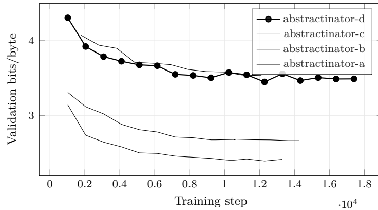
Figure 13: Bits per Byte across the 4 most recent experiments with comparable validation curves; the leading run (abstractinator-d) is drawn in bold. Generated from run logs - metrics that are not comparable across families (token loss vs. byte bits-per-byte vs. codec/CALM BrierLM) are excluded by construction, so the curves on this axis mean the same thing.
