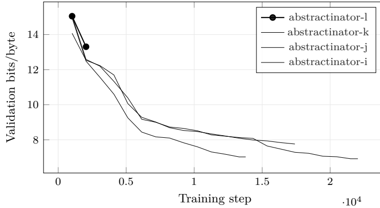
Figure 13: Bits per Byte across the 4 most recent experiments with comparable validation curves; the current experiment (abstractinator-l) is drawn in bold. Bold marks which run this build is reporting on , not which run scores best. The curves end wherever each run stopped, so they are at different points along their own training, and their endpoints are not a ranking. Generated from run logs - metrics that are not comparable across families (token loss vs. byte bits-per-byte vs. codec/CALM BrierLM) are excluded by construction, so the curves on this axis mean the same thing.
