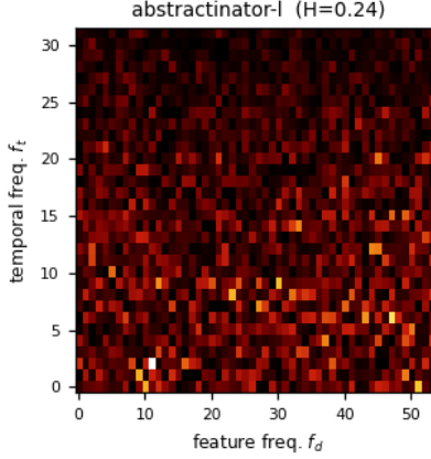
Figure 2: The static amplitude spectrum |a[f_t, f_d]| for abstractinator-l - the learned grid that, inverse-transformed through the frozen Weyl phases, becomes the bias field. This is the heatmap the text describes: energy that settles into a low-frequency band (small f_t, f_d ) is the corpus rhythm crystallizing, while a grid that stays uniform is a field still indistinguishable from noise. Hoyer concentration H = 0.24 quantifies it on the same [0, 1] scale the prose names (1 = a single cell, 0 = uniform), computed from this very tensor by concentration() - the same value the dashboard logs live. The pink 1/f^\alpha prior lives in the frozen basis, not in these amplitudes, so the grid shown is exactly what the head exposes.
