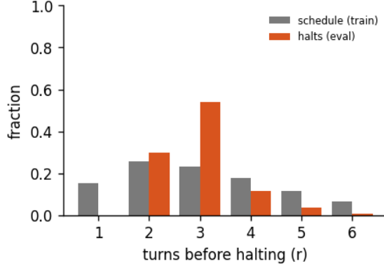
Figure 8: Halting distribution: the fraction of forward passes that stop after r turns, for the 6-turn recurrent loop of run abstractinator-1, early-halt rate 34%, mean boundary KL 0.166. schedule is the random loop-count the model trains under; halts is where the KL gate actually stops at inference. A mass pinned at the maximum (KL never collapsing) is the honest signature of a model that has not yet learned to converge early - the decision is real, not yet decisive.
