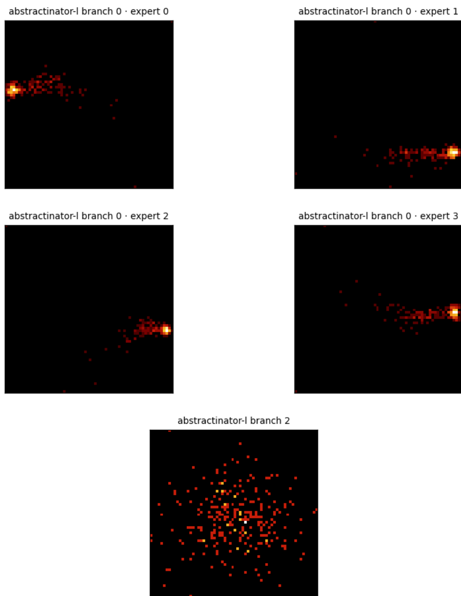
Figure 11: Center PCA density for the 5 crystal heads of abstractinator-l - a single multi-head model (prismatic4’s VEAR crystal bank), so these are that run’s own heads (branch 0 · expert 0, branch 0 · expert 1, branch 0 · expert 2, branch 0 · expert 3, branch 2), not a cross-run mix. Each panel is the top-2 PCA projection of a head’s vocabulary centers, binned to a 64 \times 64 density grid (log color) - the same snapshot the dashboard renders live. The bank’s experts settle into structurally distinct geometries - the between-expert variance the router selects over.
