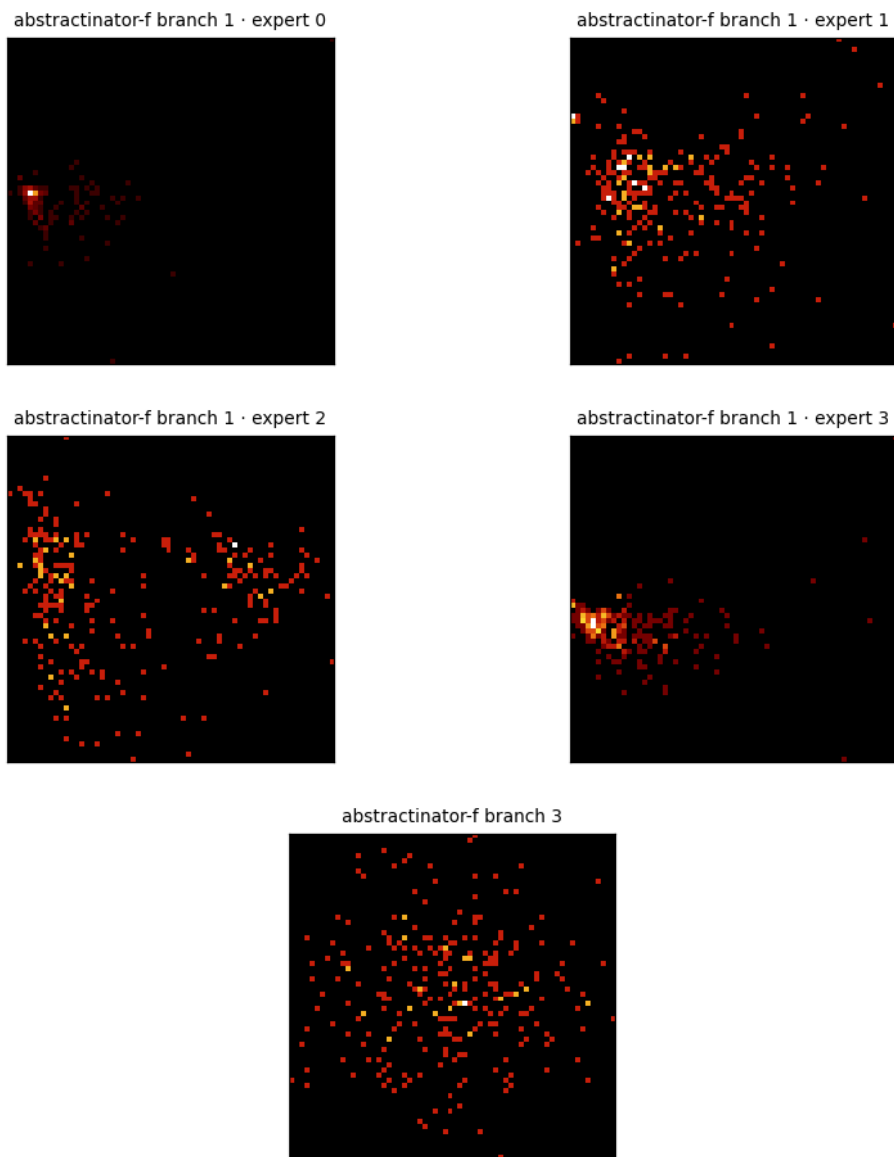
Figure 11: Center PCA density for the 5 crystal heads of abstractinator-f - a single multi-head model (prismatic4’s VEAR crystal bank), so these are that run’s own heads (branch 1 · expert 0, branch 1 · expert 1, branch 1 · expert 2, branch 1 · expert 3, branch 3), not a cross-run mix. Each panel is the top-2 PCA projection of a head’s vocabulary centers, binned to a 64 \times 64 density grid (log color) - the same snapshot the dashboard renders live. The bank’s experts settle into structurally distinct geometries - the between-expert variance the router selects over.
