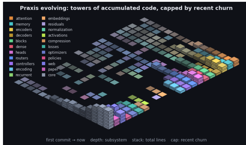
Figure 11: Praxis's git history as an isometric terrain over the last 2424 commits. Each cell is one subsystem in one time window: a stack of base blocks for its accumulated size (total lines, recency-weighted) topped by a vivid cap for that window's line churn - the standing codebase carrying the recent activity. Both are weighted by recency (the kernel the model applies to a sequence, turned on the repository): recent windows stack tall with bright caps while history thins toward the always-present prior - the low valley we roll into. Color fades from each subsystem's hue toward a neutral prior into the past, banded in phased strata over a non-linear timescale. It is the bias/variance geometry read along the frequency axis (see the project notes): loud recent corrections over the quiet, ever-present base. By recency-weighted churn the current center of gravity is core, web, paper. The framework charts the hand that builds it.
