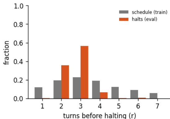
Figure 7: Halting distribution: the fraction of forward passes that stop after r turns, for the 7-turn recurrent loop of run abstractinator-c, early-halt rate 37%, mean boundary KL 0.298. schedule is the random loop-count the model trains under; halts is where the KL gate actually stops at inference. A mass pinned at the maximum (KL never collapsing) is the honest signature of a model that has not yet learned to converge early - the decision is real, not yet decisive.
