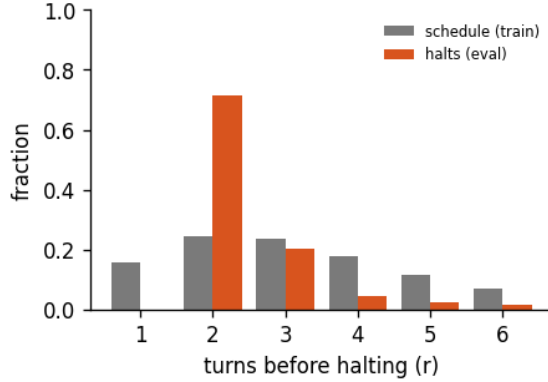
Figure 8: Halting distribution: the fraction of forward passes that stop after r turns, for the 6-turn recurrent loop of run abstractinator-j, early-halt rate 41%, mean boundary KL 0.226. schedule is the random loop-count the model trains under; halts is where the KL gate actually stops at inference. A mass pinned at the maximum (KL never collapsing) is the honest signature of a model that has not yet learned to converge early - the decision is real, not yet decisive.
