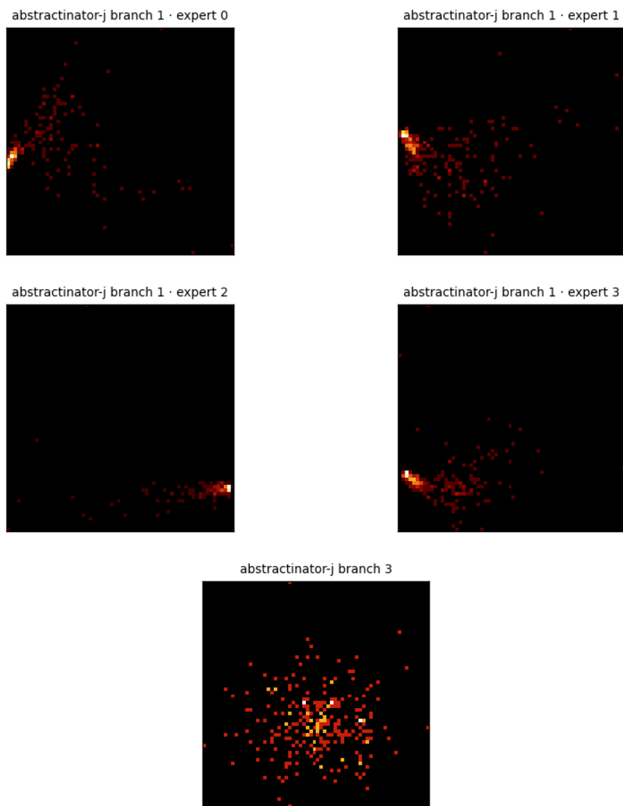
Figure 11: Center PCA density for the 5 crystal heads of abstractinator-j - a single multi-head model (prismatic4's VEAR crystal bank), so these are that run's own heads (branch 1 · expert 0, branch 1 · expert 1, branch 1 · expert 2, branch 1 · expert 3, branch 3), not a cross-run mix. Each panel is the top-2 PCA projection of a head's vocabulary centers, binned to a 64 \times 64 density grid (log color) - the same snapshot the dashboard renders live. The bank's experts settle into structurally distinct geometries - the between-expert variance the router selects over.
