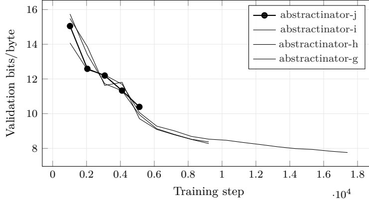
Figure 13: Bits per Byte across the 4 most recent experiments with comparable validation curves; the current experiment (abstractinator-j) is drawn in bold. Bold marks which run this build is reporting on , not which run scores best. The curves end wherever each run stopped, so they are at different points along their own training, and their endpoints are not a ranking. Generated from run logs - metrics that are not comparable across families (token loss vs. byte bits-per-byte vs. codec/CALM BrierLM) are excluded by construction, so the curves on this axis mean the same thing.
