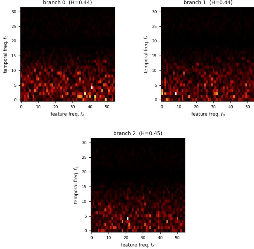
Figure 2: The static amplitude spectrum |a[f_t, f_d]| across the 3 arms of abstractinator-j’s prismatic head - the learned grid that, inverse-transformed through the frozen Weyl phases, becomes the bias field. This is the heatmap the text describes: energy that settles into a low-frequency band (small f_t, f_d ) is the corpus rhythm crystallizing, while a grid that stays uniform is a field still indistinguishable from noise. Hoyer concentrations H = 0.44, 0.44, 0.45 (left to right) quantifies it on the same [0, 1] scale the prose names (1 = a single cell, 0 = uniform), computed from this very tensor by concentration() - the same value the dashboard logs live. The pink 1/f^\alpha prior lives in the frozen basis, not in these amplitudes, so the grid shown is exactly what the head exposes.
