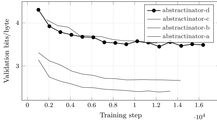
Figure 12: Bits per Byte across the 4 most recent experiments with comparable validation curves; the leading run (abstractinator-d) is drawn in bold. Generated from run logs - metrics that are not comparable across families (token loss vs. byte bits-per-byte vs. codec/CALM BrierLM) are excluded by construction, so the curves on this axis mean the same thing.
