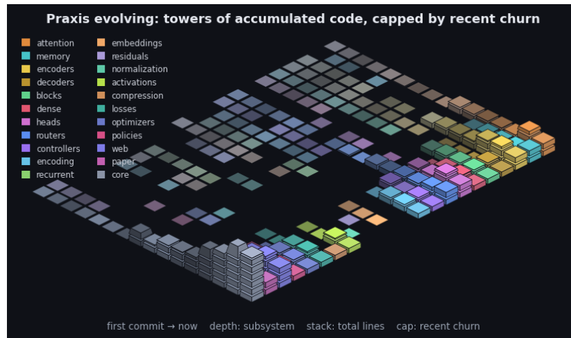
Figure 12: Praxis’s git history as an isometric terrain over the last 2607 commits. Each cell is one subsystem in one time window: a stack of base blocks for its accumulated size (total lines, recency-weighted) topped by a vivid cap for that window’s line churn - the standing codebase carrying the recent activity. Both are weighted by recency (the kernel the model applies to a sequence, turned on the repository): recent windows stack tall with bright caps while history thins toward the always-present prior - the low valley we roll into. Color fades from each subsystem’s hue toward a neutral prior into the past, banded in phased strata over a non-linear timescale. It is the bias/variance geometry read along the frequency axis (see the project notes): loud recent corrections over the quiet, ever-present base. By recency-weighted churn the current center of gravity is core, web, paper. The framework charts the hand that builds it.
