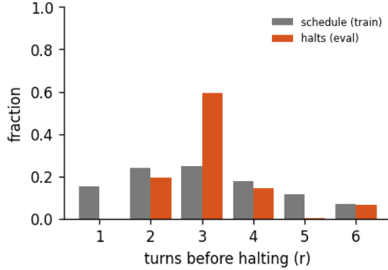
Figure 8: Halting distribution: the fraction of forward passes that stop after r turns, for the 6-turn recurrent loop of run abstractinator-h, early-halt rate 30%, mean boundary KL 0.215. schedule is the random loop-count the model trains under; halts is where the KL gate actually stops at inference. A mass pinned at the maximum (KL never collapsing) is the honest signature of a model that has not yet learned to converge early - the decision is real, not yet decisive.
