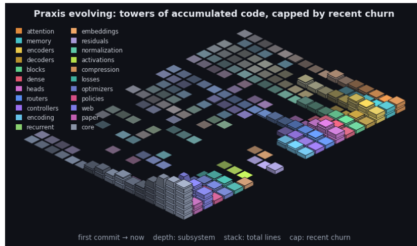
Figure 12: Praxis's git history as an isometric terrain over the last 2476 commits. Each cell is one subsystem in one time window: a stack of base blocks for its accumulated size (total lines, recency-weighted) topped by a vivid cap for that window's line churn - the standing codebase carrying the recent activity. Both are weighted by recency (the kernel the model applies to a sequence, turned on the repository): recent windows stack tall with bright caps while history thins toward the always-present prior - the low valley we roll into. Color fades from each subsystem's hue toward a neutral prior into the past, banded in phased strata over a non-linear timescale. It is the bias/variance geometry read along the frequency axis (see the project notes): loud recent corrections over the quiet, ever-present base. By recency-weighted churn the current center of gravity is core, web, paper. The framework charts the hand that builds it.
