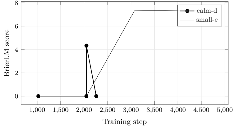
Figure 5: BrierLM across the 2 most recent experiments with comparable validation curves; the leading run (calm-d) is drawn in bold. Generated from run logs - metrics that are not comparable across families (token loss vs. byte bits-per-byte vs. codec/CALM BrierLM) are excluded by construction, so the curves on this axis mean the same thing.
