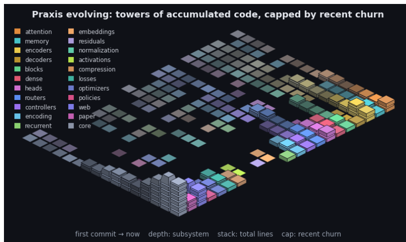
Figure 4: Praxis’s git history as an isometric terrain over the last 2276 commits. Each cell is one subsystem in one time window: a stack of base blocks for its accumulated size (total lines, recency-weighted) topped by a vivid cap for that window’s line churn - the standing codebase carrying the recent activity. Both are weighted by recency (the kernel the model applies to a sequence, turned on the repository): recent windows stack tall with bright caps while history thins toward the always-present prior - the low valley we roll into. Color fades from each subsystem’s hue toward a neutral prior into the past, banded in phased strata over a non-linear timescale. It is the bias/variance geometry read along the frequency axis (see the project notes): loud recent corrections over the quiet, ever-present base. By recency-weighted churn the current center of gravity is core, web, encoders. The framework charts the hand that builds it.
