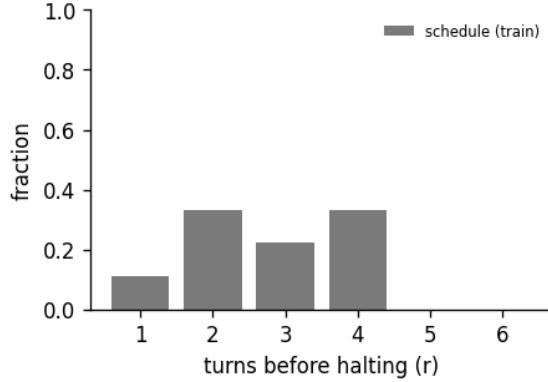
Figure 8: Halting distribution: the fraction of forward passes that stop after r turns, for the 6-turn recurrent loop of run compile-probe. schedule is the random loop-count the model trains under; halts is where the KL gate actually stops at inference. A mass pinned at the maximum (KL never collapsing) is the honest signature of a model that has not yet learned to converge early - the decision is real, not yet decisive.
