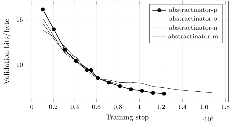
Figure 13: Bits per Byte across the 4 most recent experiments with comparable validation curves; the current experiment (abstractinator-p) is drawn in bold. Bold marks which run this build is reporting on , not which run scores best. The curves end wherever each run stopped, so they are at different points along their own training, and their endpoints are not a ranking. Generated from run logs - metrics that are not comparable across families (token loss vs. byte bits-per-byte vs. codec/CALM BrierLM) are excluded by construction, so the curves on this axis mean the same thing.
