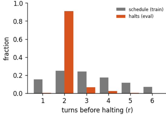
Figure 8: Halting distribution: the fraction of forward passes that stop after r turns, for the 6-turn recurrent loop of run abstractinator-e, early-halt rate 47%, mean boundary KL 0.685. schedule is the random loop-count the model trains under; halts is where the KL gate actually stops at inference. A mass pinned at the maximum (KL never collapsing) is the honest signature of a model that has not yet learned to converge early - the decision is real, not yet decisive.
