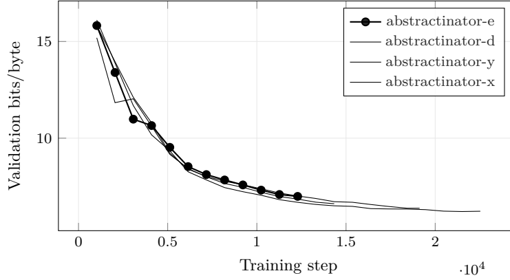
Figure 13: Bits per Byte across the 4 most recent experiments with comparable validation curves; the current experiment (abstractinator-e) is drawn in bold. Bold marks which run this build is reporting on , not which run scores best. The curves end wherever each run stopped, so they are at different points along their own training, and their endpoints are not a ranking. Generated from run logs - metrics that are not comparable across families (token loss vs. byte bits-per-byte vs. codec/CALM BrierLM) are excluded by construction, so the curves on this axis mean the same thing.
