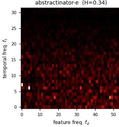
Figure 2: The static amplitude spectrum |a[f_t, f_d]| for abstractinator-e - the learned grid that, inverse-transformed through the frozen Weyl phases, becomes the bias field. This is the heatmap the text describes: energy that settles into a low-frequency band (small f_t, f_d ) is the corpus rhythm crystallizing, while a grid that stays uniform is a field still indistinguishable from noise. Hoyer concentration H = 0.34 quantifies it on the same [0, 1] scale the prose names (1 = a single cell, 0 = uniform), computed from this very tensor by concentration() - the same value the dashboard logs live. The pink 1/f^\alpha prior lives in the frozen basis, not in these amplitudes, so the grid shown is exactly what the head exposes.
