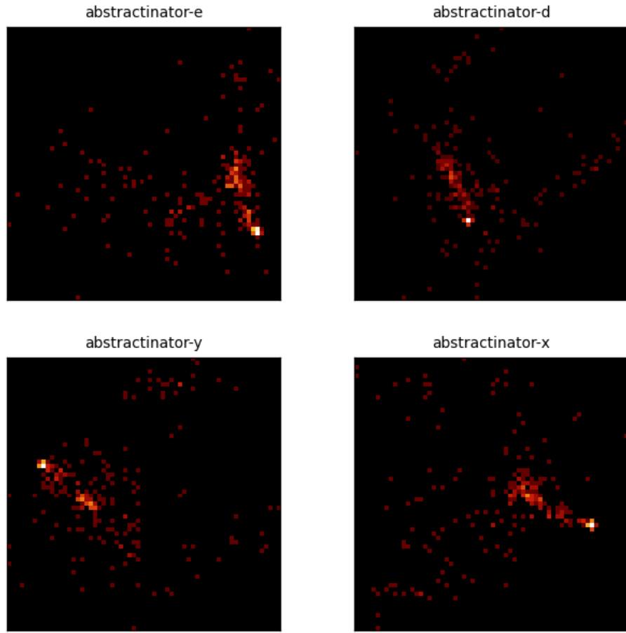
Figure 11: Center PCA density for the 4 most recent crystal-head runs (abstractinator-e, abstractinator-d, abstractinator-y, abstractinator-x). Each panel is the top-2 PCA projection of a head’s vocabulary centers, binned to a 64 \times 64 density grid (log color) - the same snapshot the dashboard renders live. Different runs settle into structurally different geometries, not noise.
