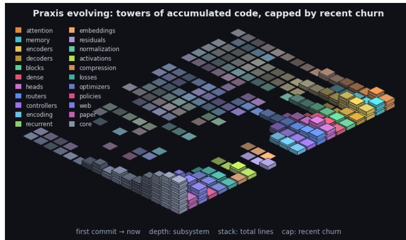
Figure 12: Praxis’s git history as an isometric terrain over the last 2550 commits. Each cell is one subsystem in one time window: a stack of base blocks for its accumulated size (total lines, recency-weighted) topped by a vivid cap for that window’s line churn - the standing codebase carrying the recent activity. Both are weighted by recency (the kernel the model applies to a sequence, turned on the repository): recent windows stack tall with bright caps while history thins toward the always-present prior - the low valley we roll into. Color fades from each subsystem’s hue toward a neutral prior into the past, banded in phased strata over a non-linear timescale. It is the bias/variance geometry read along the frequency axis (see the project notes): loud recent corrections over the quiet, ever-present base. By recency-weighted churn the current center of gravity is core, web, paper. The framework charts the hand that builds it.
