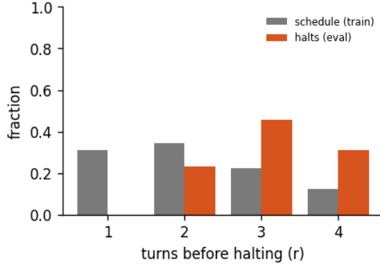
Figure 7: Halting distribution: the fraction of forward passes that stop after r turns, for the 4-turn recurrent loop of run abstractinator-e, early-halt rate 25%, mean boundary KL 0.454. schedule is the random loop-count the model trains under; halts is where the KL gate actually stops at inference. A mass pinned at the maximum (KL never collapsing) is the honest signature of a model that has not yet learned to converge early - the decision is real, not yet decisive.
