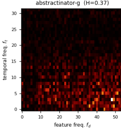
Figure 2: The static amplitude spectrum |a[f_t, f_d]| for abstractinator-g - the learned grid that, inverse-transformed through the frozen Weyl phases, becomes the bias field. This is the heatmap the text describes: energy that settles into a low-frequency band (small f_t, f_d ) is the corpus rhythm crystallizing, while a grid that stays uniform is a field still indistinguishable from noise. Hoyer concentration H = 0.37 quantifies it on the same [0, 1] scale the prose names (1 = a single cell, 0 = uniform), computed from this very tensor by concentration() - the same value the dashboard logs live. The pink 1/f^\alpha prior lives in the frozen basis, not in these amplitudes, so the grid shown is exactly what the head exposes.
