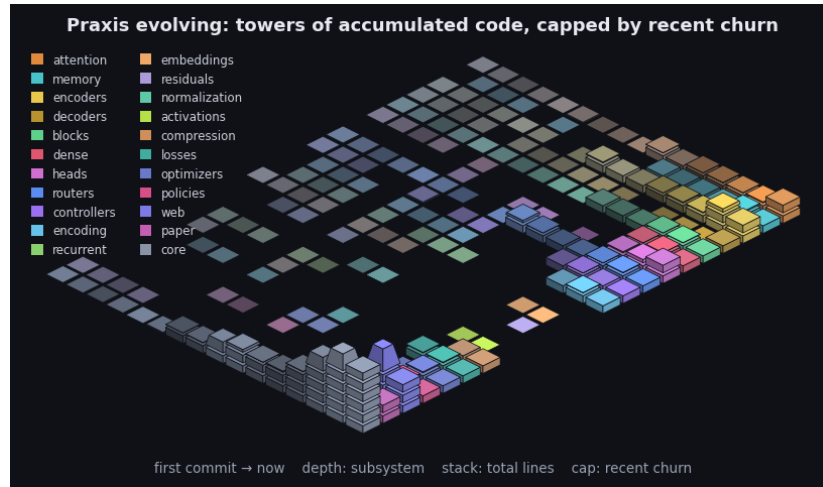
Figure 10: Praxis’s git history as an isometric terrain over the last 2395 commits. Each cell is one subsystem in one time window: a stack of base blocks for its accumulated size (total lines, recency-weighted) topped by a vivid cap for that window’s line churn - the standing codebase carrying the recent activity. Both are weighted by recency (the kernel the model applies to a sequence, turned on the repository): recent windows stack tall with bright caps while history thins toward the always-present prior - the low valley we roll into. Color fades from each subsystem’s hue toward a neutral prior into the past, banded in phased strata over a non-linear timescale. It is the bias/variance geometry read along the frequency axis (see the project notes): loud recent corrections over the quiet, ever-present base. By recency-weighted churn the current center of gravity is core, web, paper. The framework charts the hand that builds it.
