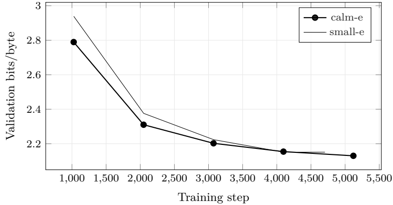
Figure 8: Bits per Byte across the 2 most recent experiments with comparable validation curves; the leading run (calm-e) is drawn in bold. Generated from run logs - metrics that are not comparable across families (token loss vs. byte bits-per-byte vs. codec/CALM BrierLM) are excluded by construction, so the curves on this axis mean the same thing.
