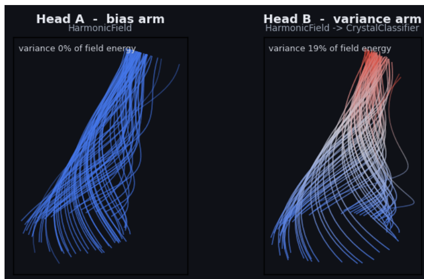
Figure 4: The prismatic head's two arms, rendered exactly as the dashboard's bias/variance strand card. Each hair is one feature, morphing from a ring (its static-eld phase) out to its (bias, variance) position with a helical twist; color runs blue (pure bias) to red (pure variance). Head A (left) is the bias arm: it reads a static eld, so every hair stays blue - a constant structural vote. Head B (right) is the variance arm, whose input-conditional envelope lets hairs swing toward red - the data-dependent vote. Each panel's subtitle lists that arm's head stack. The two together are the orthogonal bias/variance decomposition made architectural - convex and radial from the center, chaotic in the arms.
