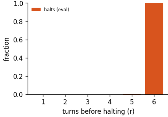
Figure 5: Halting distribution: the fraction of forward passes that stop after r turns, for the 6-turn recurrent loop of run calm-d, early-halt rate 0%, mean boundary KL 3.24. schedules is the random loop-count the model trains under; halts is where the KL gate actually stops at inference. A mass pinned at the maximum (KL never collapsing) is the honest signature of a model that has not yet learned to converge early - the decision is real, not yet decisive.
