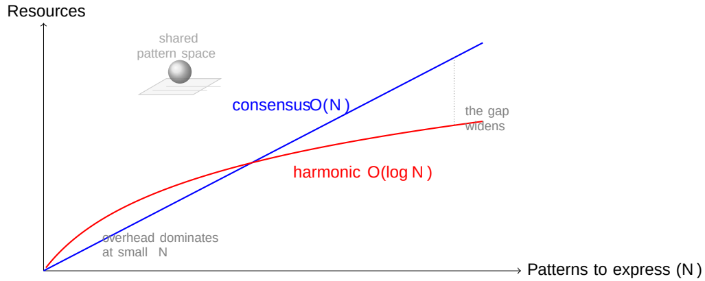
Figure 6: Conjectured scaling regimes. To express N patterns, consensus modeling - learning the mean - spends resources growing linearly in N (blue). Harmonic modeling composes patterns by interference, and K \sim \log N components suffice, so its cost grows logarithmically (red). The harmonic basis carries fixed overhead, so it loses at small N and wins at scale, where the gap widens without bound. Both must ultimately represent the same target (the shared pattern space, top); the claim is about the cost of getting there, not the destination. This figure states a conjecture, and replaces the speculative measured-curve figure of earlier drafts.
