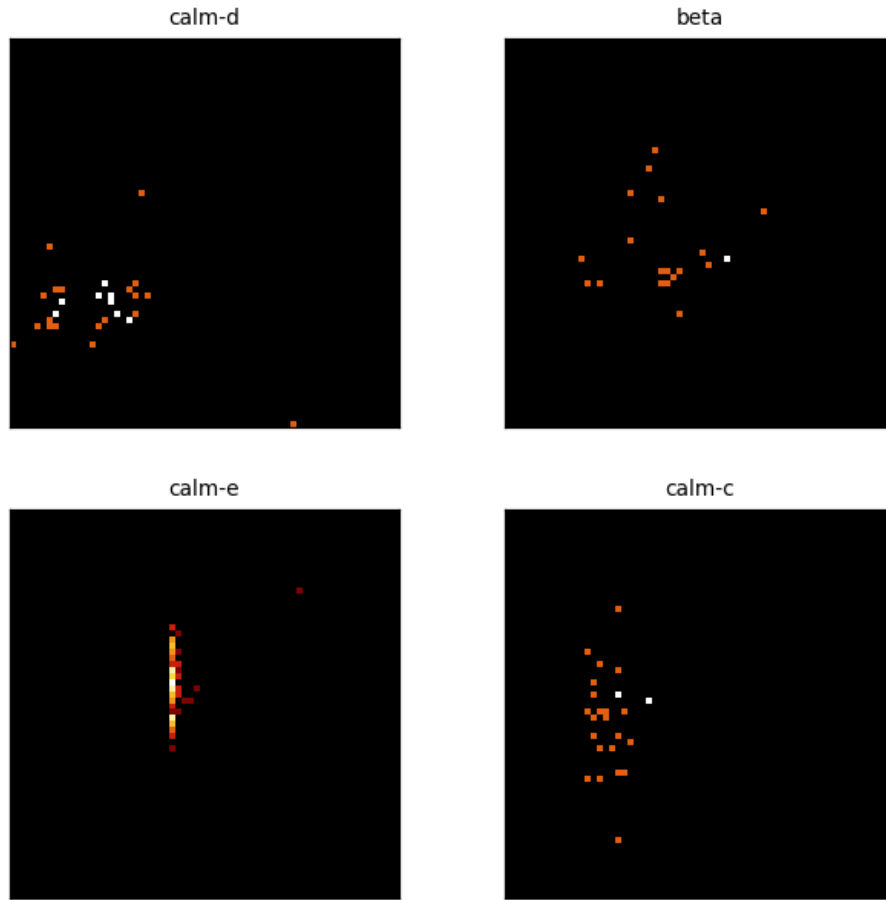
Figure 2: Center PCA density for the 4 most recent crystal-head runs (calm-d, beta, calm-e, calm-c). Each panel is the top-2 PCA projection of a head's vocabulary centers, binned to a 64 64 density grid (log color) - the same snapshot the dashboard renders live. Different runs settle into structurally different geometries, not noise.
