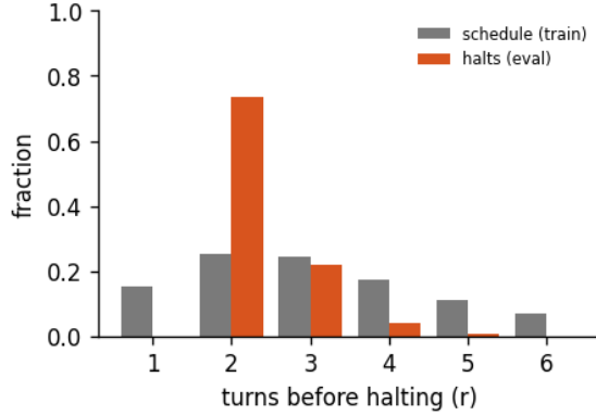
Figure 9: Halting distribution: the fraction of forward passes that stop after r turns, for the 6-turn recurrent loop of run abstractinator-x, early-halt rate 43%, mean boundary KL 1.12. schedule is the random loop-count the model trains under; halts is where the KL gate actually stops at inference. A mass pinned at the maximum (KL never collapsing) is the honest signature of a model that has not yet learned to converge early - the decision is real, not yet decisive.
