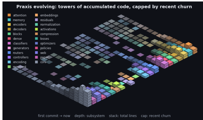
Figure 13: Praxis’s git history as an isometric terrain over the last 2618 commits. Each cell is one subsystem in one time window: a stack of base blocks for its accumulated size (total lines, recency-weighted) topped by a vivid cap for that window’s line churn - the standing codebase carrying the recent activity. Both are weighted by recency (the kernel the model applies to a sequence, turned on the repository): recent windows stack tall with bright caps while history thins toward the always-present prior - the low valley we roll into. Color fades from each subsystem’s hue toward a neutral prior into the past, banded in phased strata over a non-linear timescale. It is the bias/variance geometry read along the frequency axis (see the project notes): loud recent corrections over the quiet, ever-present base. By recency-weighted churn the current center of gravity is core, web, encoders. The framework charts the hand that builds it.
