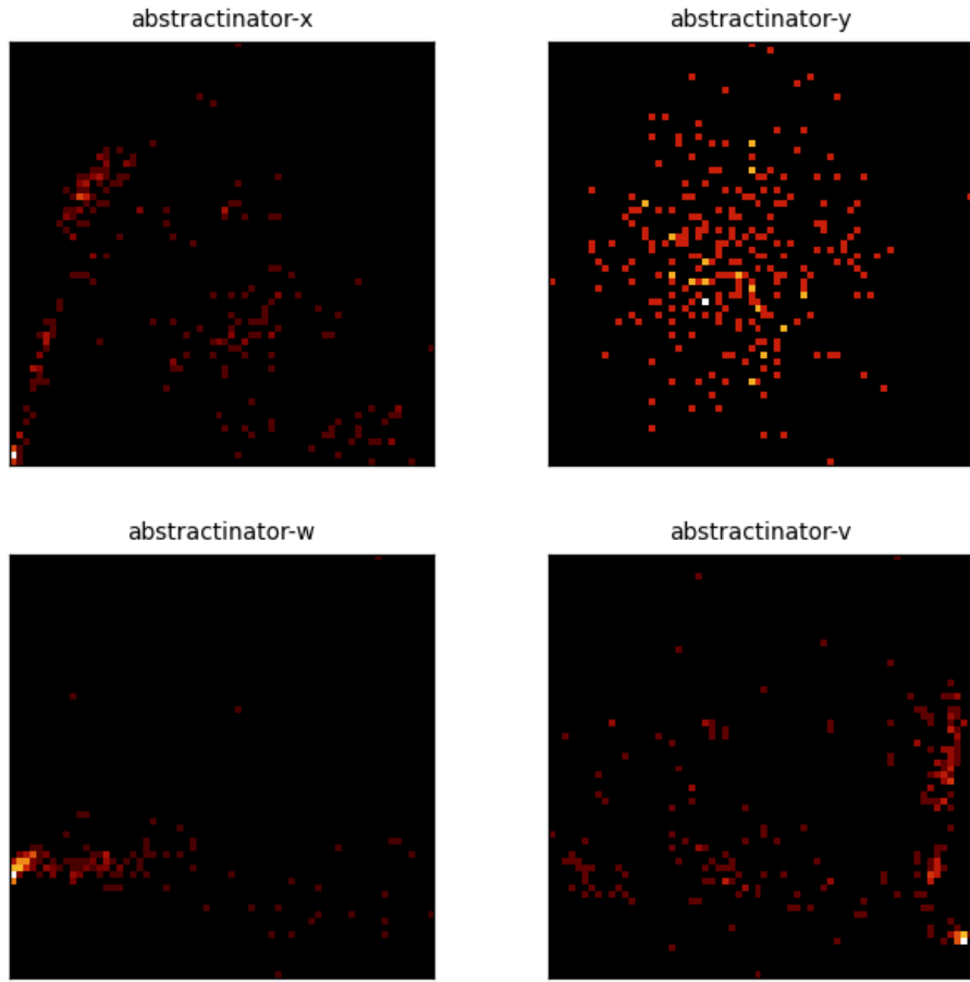
Figure 5: Center PCA density for the 4 most recent crystal-head runs (abstractinator-x, abstractinator-y, abstractinator-w, abstractinator-v). Each panel is the top-2 PCA projection of a head’s vocabulary centers, binned to a 64 \times 64 density grid (log color) - the same snapshot the dashboard renders live. Different runs settle into structurally different geometries, not noise.
