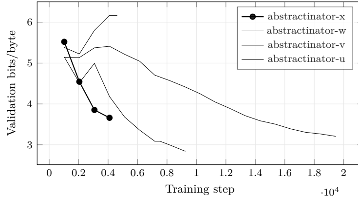
Figure 14: Bits per Byte across the 4 most recent experiments with comparable validation curves; the current experiment (abstractinator-x) is drawn in bold. Bold marks which run this build is reporting on , not which run scores best. The curves end wherever each run stopped, so they are at different points along their own training, and their endpoints are not a ranking. Generated from run logs - metrics that are not comparable across families (token loss vs. byte bits-per-byte vs. codec/CALM BrierLM) are excluded by construction, so the curves on this axis mean the same thing.
