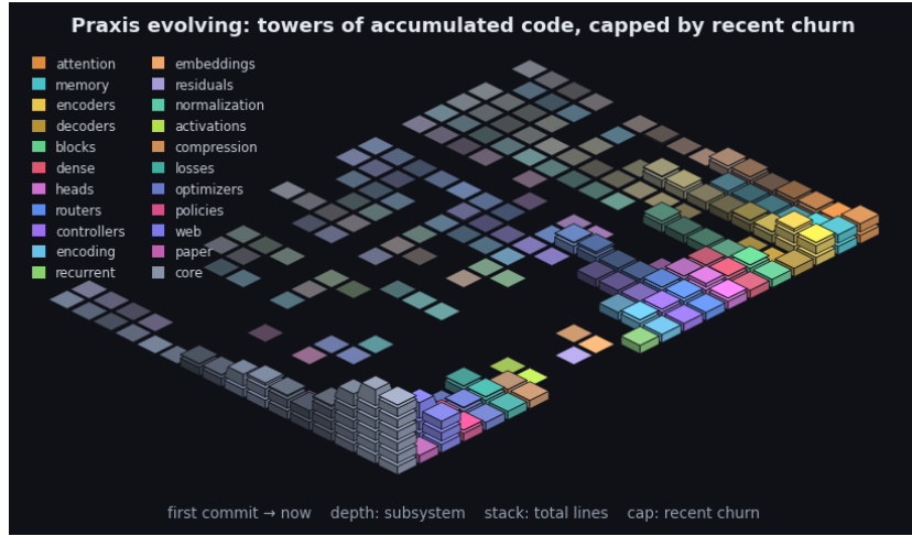
Figure 5: Praxis’s git history as an isometric terrain over the last 2238 commits. Each cell is one subsystem in one time window: a stack of base blocks for its accumulated size (total lines, recency-weighted) topped by a vivid cap for that window’s line churn - the standing codebase carrying the recent activity. Both are weighted by recency (the kernel the model applies to a sequence, turned on the repository): recent windows stack tall with bright caps while history thins toward the always-present prior - the low valley we roll into. Color fades from each subsystem’s hue toward a neutral prior into the past, banded in phased strata over a non-linear timescale. It is the bias/variance geometry read along the frequency axis (see the project notes): loud recent corrections over the quiet, ever-present base. By recency-weighted churn the current center of gravity is core, web, encoders. The framework charts the hand that builds it.
