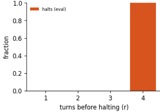
Figure 3: Halting distribution: the fraction of forward passes that stop after r turns, for the 4-turn recurrent loop of run calm-f, early-halt rate 0%, mean boundary KL 4.11. schedule is the random loop-count the model trains under; halts is where the KL gate actually stops at inference. A mass pinned at the maximum (KL never collapsing) is the honest signature of a model that has not yet learned to converge early - the decision is real, not yet decisive.
