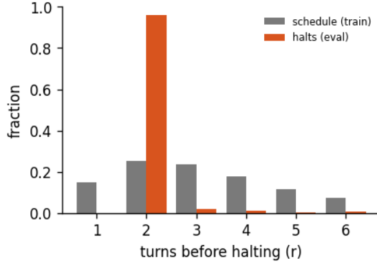
Figure 9: Halting distribution: the fraction of forward passes that stop after r turns, for the 6-turn recurrent loop of run abstractinator-p, early-halt rate 48%, mean boundary KL 1.57. schedule is the random loop-count the model trains under; halts is where the KL gate actually stops at inference. A mass pinned at the maximum (KL never collapsing) is the honest signature of a model that has not yet learned to converge early - the decision is real, not yet decisive.
