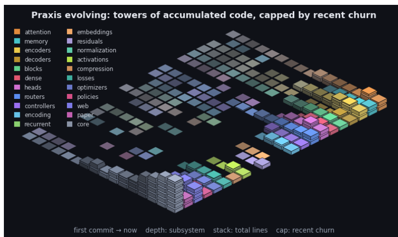
Figure 13: Praxis’s git history as an isometric terrain over the last 2582 commits. Each cell is one subsystem in one time window: a stack of base blocks for its accumulated size (total lines, recency-weighted) topped by a vivid cap for that window’s line churn - the standing codebase carrying the recent activity. Both are weighted by recency (the kernel the model applies to a sequence, turned on the repository): recent windows stack tall with bright caps while history thins toward the always-present prior - the low valley we roll into. Color fades from each subsystem’s hue toward a neutral prior into the past, banded in phased strata over a non-linear timescale. It is the bias/variance geometry read along the frequency axis (see the project notes): loud recent corrections over the quiet, ever-present base. By recency-weighted churn the current center of gravity is core, web, paper. The framework charts the hand that builds it.
