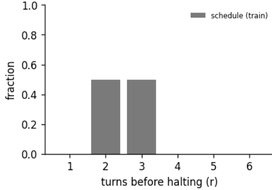
Figure 9: Halting distribution: the fraction of forward passes that stop after r turns, for the 6-turn recurrent loop of run abstractinator-q. schedule is the random loop-count the model trains under; halts is where the KL gate actually stops at inference. A mass pinned at the maximum (KL never collapsing) is the honest signature of a model that has not yet learned to converge early - the decision is real, not yet decisive.
