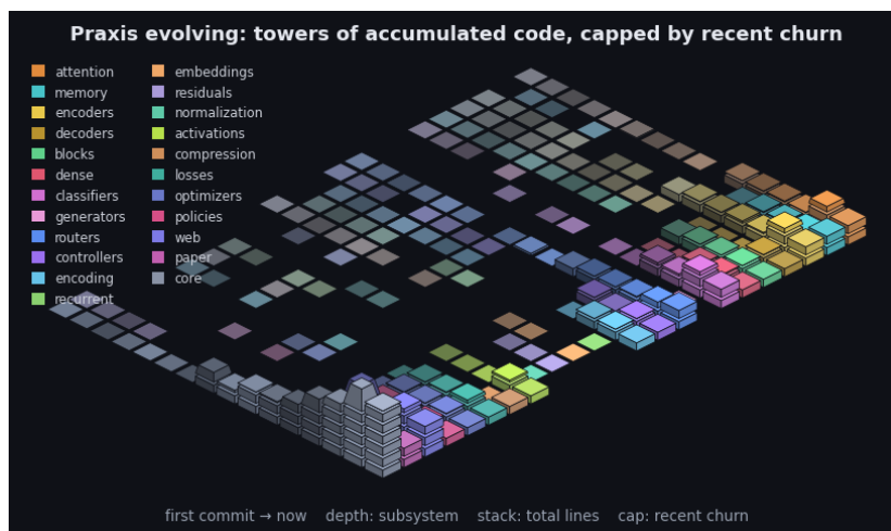
Figure 9: Praxis’s git history as an isometric terrain over the last 2665 commits. Each cell is one subsystem in one time window: a stack of base blocks for its accumulated size (total lines, recency-weighted) topped by a vivid cap for that window’s line churn - the standing codebase carrying the recent activity. Both are weighted by recency (the kernel the model applies to a sequence, turned on the repository): recent windows stack tall with bright caps while history thins toward the always-present prior - the low valley we roll into. Color fades from each subsystem’s hue toward a neutral prior into the past, banded in phased strata over a non-linear timescale. It is the bias/variance geometry read along the frequency axis (see the project notes): loud recent corrections over the quiet, ever-present base. By recency-weighted churn the current center of gravity is core, web, encoders. The framework charts the hand that builds it.
