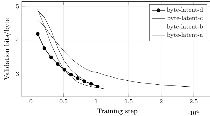
Figure 10: Bits per Byte across the 4 most recent experiments with comparable validation curves; the current experiment (byte-latent-d) is drawn in bold. Bold marks which run this build is reporting on , not which run scores best. The curves end wherever each run stopped, so they are at different points along their own training, and their endpoints are not a ranking. Generated from run logs - metrics that are not comparable across families (token loss vs. byte bits-per-byte vs. codec/CALM BrierLM) are excluded by construction, so the curves on this axis mean the same thing.
