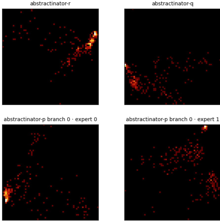
Figure 11: Center PCA density for the 4 most recent crystal-head runs (abstractinator-r, abstractinator-q, abstractinator-p (branch 0 · expert 0), abstractinator-p (branch 0 · expert 1)). Each panel is the top-2 PCA projection of a head’s vocabulary centers, binned to a 64 \times 64 density grid (log color) - the same snapshot the dashboard renders live. Different runs settle into structurally different geometries, not noise.
