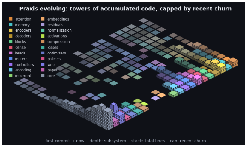
Figure 4: Praxis’s git history as an isometric terrain over the last 2323 commits. Each cell is one subsystem in one time window: a stack of base blocks for its accumulated size (total lines, recency-weighted) topped by a vivid cap for that window’s line churn - the standing codebase carrying the recent activity. Both are weighted by recency (the kernel the model applies to a sequence, turned on the repository): recent windows stack tall with bright caps while history thins toward the always-present prior - the low valley we roll into. Color fades from each subsystem’s hue toward a neutral prior into the past, banded in phased strata over a non-linear timescale. It is the bias/variance geometry read along the frequency axis (see the project notes): loud recent corrections over the quiet, ever-present base. By recency-weighted churn the current center of gravity is core, web, paper. The framework charts the hand that builds it.
