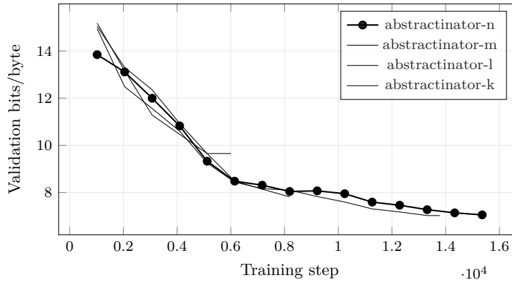
Figure 13: Bits per Byte across the 4 most recent experiments with comparable validation curves; the current experiment (abstractinator-n) is drawn in bold. Bold marks which run this build is reporting on , not which run scores best. The curves end wherever each run stopped, so they are at different points along their own training, and their endpoints are not a ranking. Generated from run logs - metrics that are not comparable across families (token loss vs. byte bits-per-byte vs. codec/CALM BrierLM) are excluded by construction, so the curves on this axis mean the same thing.
