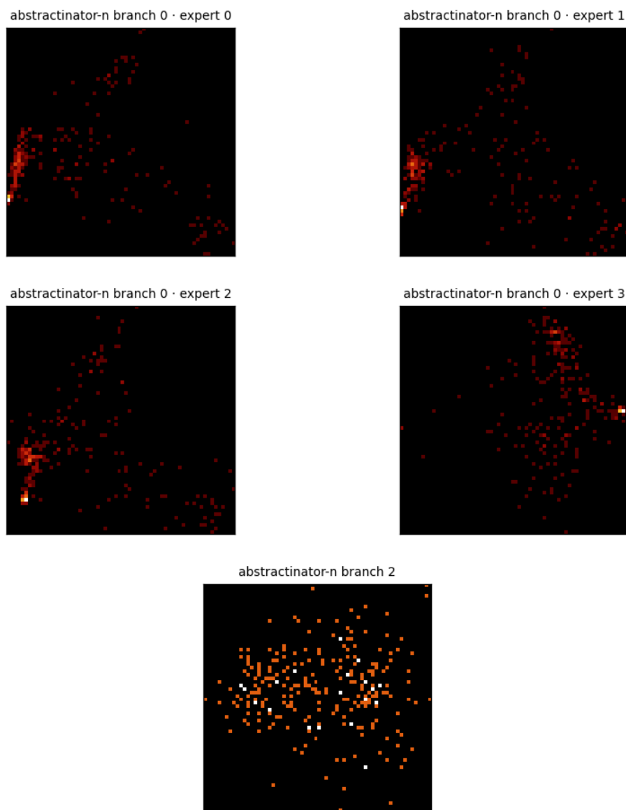
Figure 11: Center PCA density for the 5 crystal heads of abstractinator-n - a single multi-head model (prismatic4’s VEAR crystal bank), so these are that run’s own heads (branch 0 · expert 0, branch 0 · expert 1, branch 0 · expert 2, branch 0 · expert 3, branch 2), not a cross-run mix. Each panel is the top-2 PCA projection of a head’s vocabulary centers, binned to a 64 \times 64 density grid (log color) - the same snapshot the dashboard renders live. The bank’s experts settle into structurally distinct geometries - the between-expert variance the router selects over.
