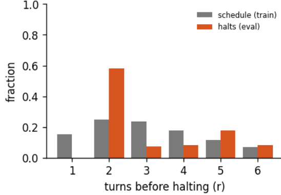
Figure 8: Halting distribution: the fraction of forward passes that stop after r turns, for the 6-turn recurrent loop of run abstractinator-n, early-halt rate 30%, mean boundary KL 0.517. schedule is the random loop-count the model trains under; halts is where the KL gate actually stops at inference. A mass pinned at the maximum (KL never collapsing) is the honest signature of a model that has not yet learned to converge early - the decision is real, not yet decisive.
