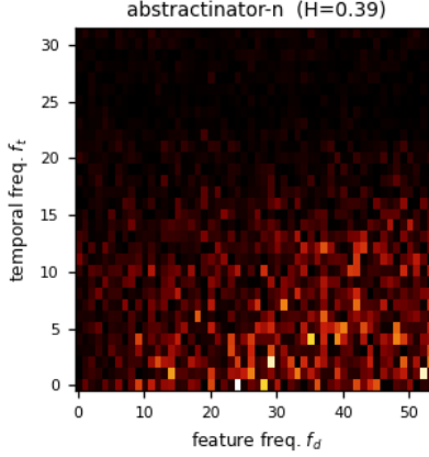
Figure 2: The static amplitude spectrum |a[f_t, f_d]| for abstractinator-n - the learned grid that, inverse-transformed through the frozen Weyl phases, becomes the bias field. This is the heatmap the text describes: energy that settles into a low-frequency band (small f_t, f_d ) is the corpus rhythm crystallizing, while a grid that stays uniform is a field still indistinguishable from noise. Hoyer concentration H = 0.39 quantifies it on the same [0, 1] scale the prose names (1 = a single cell, 0 = uniform), computed from this very tensor by concentration() - the same value the dashboard logs live. The pink 1/f^\alpha prior lives in the frozen basis, not in these amplitudes, so the grid shown is exactly what the head exposes.
