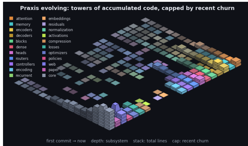
Figure 10: Praxis's git history as an isometric terrain over the last 2389 commits. Each cell is one subsystem in one time window: a stack of base blocks for its accumulated size (total lines, recency-weighted) topped by a vivid cap for that window's line churn - the standing codebase carrying the recent activity. Both are weighted by recency (the kernel the model applies to a sequence, turned on the repository): recent windows stack tall with bright caps while history thins toward the always-present prior - the low valley we roll into. Color fades from each subsystem's hue toward a neutral prior into the past, banded in phased strata over a non-linear timescale. It is the bias/variance geometry read along the frequency axis (see the project notes): loud recent corrections over the quiet, ever-present base. By recency-weighted churn the current center of gravity is core, web, paper. The framework charts the hand that builds it.
