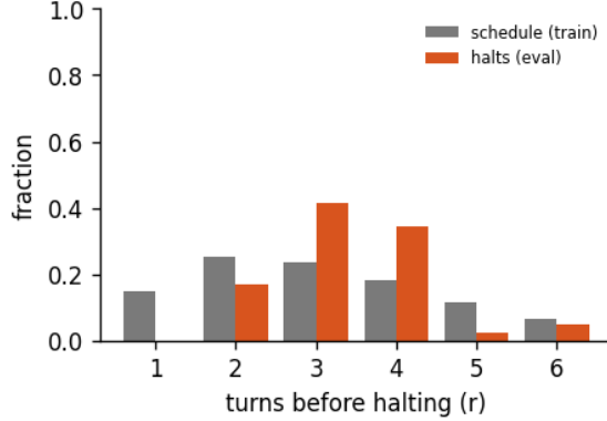
Figure 8: Halting distribution: the fraction of forward passes that stop after r turns, for the 6-turn recurrent loop of run abstractinator-1, early-halt rate 29%, mean boundary KL 0.243. schedule is the random loop-count the model trains under; halts is where the KL gate actually stops at inference. A mass pinned at the maximum (KL never collapsing) is the honest signature of a model that has not yet learned to converge early - the decision is real, not yet decisive.
