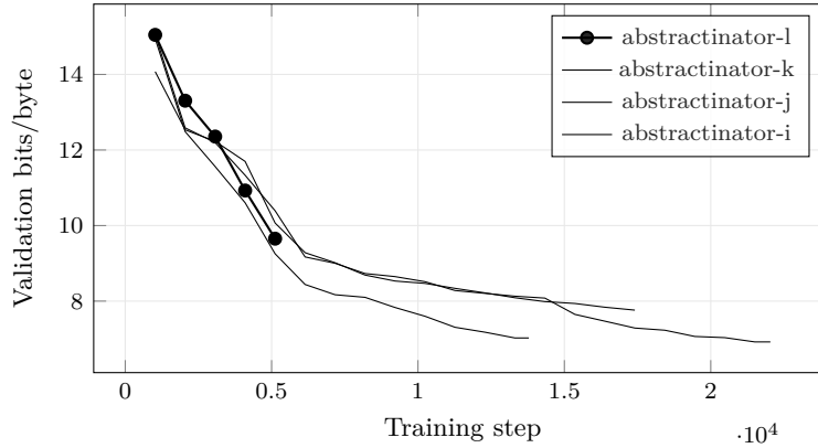
Figure 13: Bits per Byte across the 4 most recent experiments with comparable validation curves; the current experiment ( abstractinator-l ) is drawn in bold. Bold marks which run this build is reporting on , not which run scores best. The curves end wherever each run stopped, so they are at different points along their own training, and their endpoints are not a ranking. Generated from run logs - metrics that are not comparable across families (token loss vs. byte bits-per-byte vs. codec/CALM BrierLM) are excluded by construction, so the curves on this axis mean the same thing.
