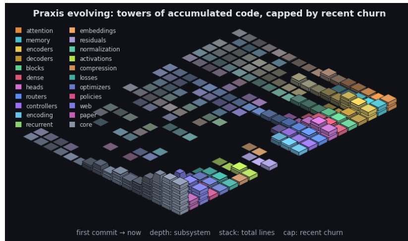
Figure 12: Praxis’s git history as an isometric terrain over the last 2505 commits. Each cell is one subsystem in one time window: a stack of base blocks for its accumulated size (total lines, recency-weighted) topped by a vivid cap for that window’s line churn - the standing codebase carrying the recent activity. Both are weighted by recency (the kernel the model applies to a sequence, turned on the repository): recent windows stack tall with bright caps while history thins toward the always-present prior - the low valley we roll into. Color fades from each subsystem’s hue toward a neutral prior into the past, banded in phased strata over a non-linear timescale. It is the bias/variance geometry read along the frequency axis (see the project notes): loud recent corrections over the quiet, ever-present base. By recency-weighted churn the current center of gravity is core, web, paper. The framework charts the hand that builds it.
