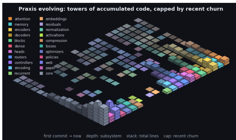
Figure 4: Praxis’s git history as an isometric terrain over the last 2295 commits. Each cell is one subsystem in one time window: a stack of base blocks for its accumulated size (total lines, recency-weighted) topped by a vivid cap for that window’s line churn - the standing codebase carrying the recent activity. Both are weighted by recency (the kernel the model applies to a sequence, turned on the repository): recent windows stack tall with bright caps while history thins toward the always-present prior - the low valley we roll into. Color fades from each subsystem’s hue toward a neutral prior into the past, banded in phased strata over a non-linear timescale. It is the bias/variance geometry read along the frequency axis (see the project notes): loud recent corrections over the quiet, ever-present base. By recency-weighted churn the current center of gravity is core, web, paper. The framework charts the hand that builds it.
