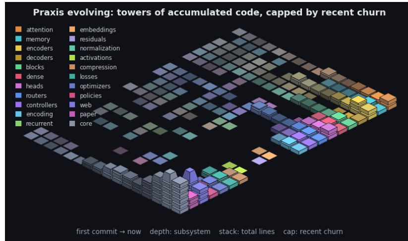
Figure 10: Praxis's git history as an isometric terrain over the last 2371 commits. Each cell is one subsystem in one time window: a stack of base blocks for its accumulated size (total lines, recency-weighted) topped by a vivid cap for that window's line churn - the standing codebase carrying the recent activity. Both are weighted by recency (the kernel the model applies to a sequence, turned on the repository): recent windows stack tall with bright caps while history thins toward the always-present prior - the low valley we roll into. Color fades from each subsystem's hue toward a neutral prior into the past, banded in phased strata over a non-linear timescale. It is the bias/variance geometry read along the frequency axis (see the project notes): loud recent corrections over the quiet, ever-present base. By recency-weighted churn the current center of gravity is core, web, paper. The framework charts the hand that builds it.
