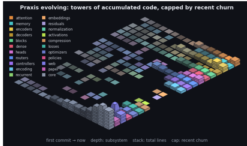
Figure 10: Praxis's git history as an isometric terrain over the last 2390 commits. Each cell is one subsystem in one time window: a stack of base blocks for its accumulated size (total lines, recency-weighted) topped by a vivid cap for that window's line churn - the standing codebase carrying the recent activity. Both are weighted by recency (the kernel the model applies to a sequence, turned on the repository): recent windows stack tall with bright caps while history thins toward the always-present prior - the low valley we roll into. Color fades from each subsystem's hue toward a neutral prior into the past, banded in phased strata over a non-linear timescale. It is the bias/variance geometry read along the frequency axis (see the project notes): loud recent corrections over the quiet, ever-present base. By recency-weighted churn the current center of gravity is core, web, paper. The framework charts the hand that builds it.
