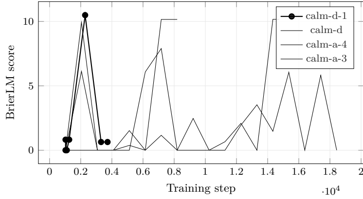
Figure 6: BrierLM across the 4 most recent experiments with comparable validation curves; the leading run (calm-d-1) is drawn in bold. Generated from run logs - metrics that are not comparable across families (token loss vs. byte bits-per-byte vs. codec/CALM BrierLM) are excluded by construction, so the curves on this axis mean the same thing.
