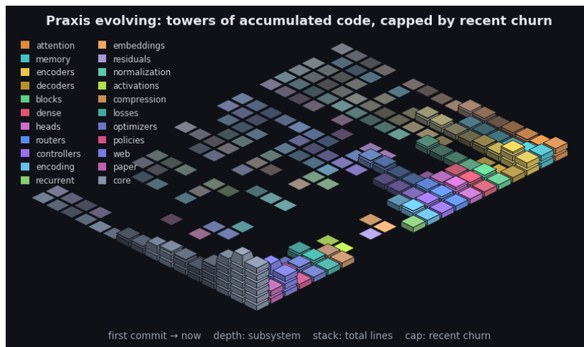
Figure 4: Praxis’s git history as an isometric terrain over the last 2255 commits. Each cell is one subsystem in one time window: a stack of base blocks for its accumulated size (total lines, recency-weighted) topped by a vivid cap for that window’s line churn - the standing codebase carrying the recent activity. Both are weighted by recency (the kernel the model applies to a sequence, turned on the repository): recent windows stack tall with bright caps while history thins toward the always-present prior - the low valley we roll into. Color fades from each subsystem’s hue toward a neutral prior into the past, banded in phased strata over a non-linear timescale. It is the bias/variance geometry read along the frequency axis (see the project notes): loud recent corrections over the quiet, ever-present base. By recency-weighted churn the current center of gravity is core, web, encoders. The framework charts the hand that builds it.
