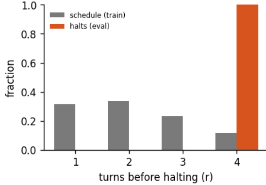
Figure 2: Halting distribution: the fraction of forward passes that stop after r turns, for the 4-turn recurrent loop of run calm-e, early-halt rate 0%, mean boundary KL 46.2. schedule is the random loop-count the model trains under; halts is where the KL gate actually stops at inference. A mass pinned at the maximum (KL never collapsing) is the honest signature of a model that has not yet learned to converge early - the decision is real, not yet decisive.
