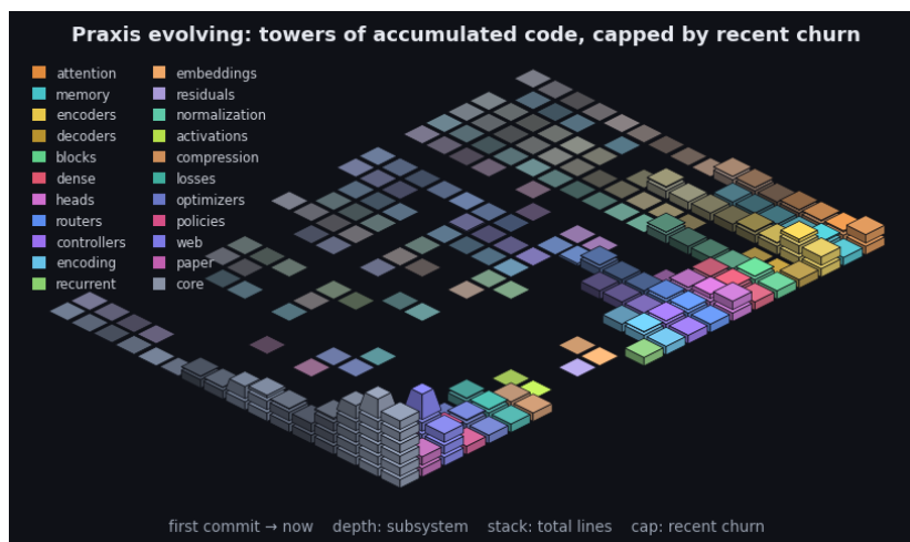
Figure 4: Praxis’s git history as an isometric terrain over the last 2325 commits. Each cell is one subsystem in one time window: a stack of base blocks for its accumulated size (total lines, recency-weighted) topped by a vivid cap for that window’s line churn - the standing codebase carrying the recent activity. Both are weighted by recency (the kernel the model applies to a sequence, turned on the repository): recent windows stack tall with bright caps while history thins toward the always-present prior - the low valley we roll into. Color fades from each subsystem’s hue toward a neutral prior into the past, banded in phased strata over a non-linear timescale. It is the bias/variance geometry read along the frequency axis (see the project notes): loud recent corrections over the quiet, ever-present base. By recency-weighted churn the current center of gravity is core, web, paper. The framework charts the hand that builds it.
