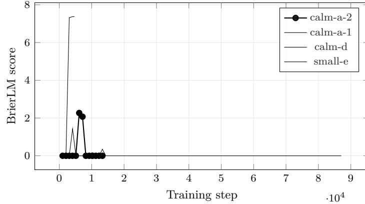
Figure 5: BrierLM across the 4 most recent experiments with comparable validation curves; the leading run (calm-a-2) is drawn in bold. Generated from run logs - metrics that are not comparable across families (token loss vs. byte bits-per-byte vs. codec/CALM BrierLM) are excluded by construction, so the curves on this axis mean the same thing.
