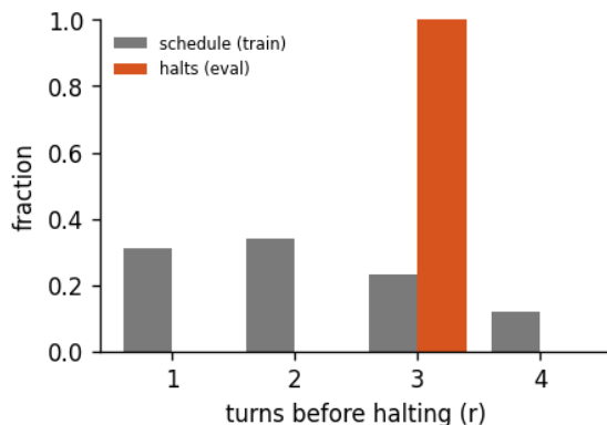
Figure 2: Halting distribution: the fraction of forward passes that stop after r turns, for the 4-turn recurrent loop of run calm-d-1, early-halt rate 33%, mean boundary KL 0.204. schedule is the random loop-count the model trains under; halts is where the KL gate actually stops at inference. A mass pinned at the maximum (KL never collapsing) is the honest signature of a model that has not yet learned to converge early - the decision is real, not yet decisive.
