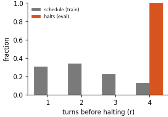
Figure 5: Halting distribution: the fraction of forward passes that stop after r turns, for the 4-turn recurrent loop of run calm-e, early-halt rate 0%, mean boundary KL 101. schedule is the random loop-count the model trains under; halts is where the KL gate actually stops at inference. A mass pinned at the maximum (KL never collapsing) is the honest signature of a model that has not yet learned to converge early - the decision is real, not yet decisive.
