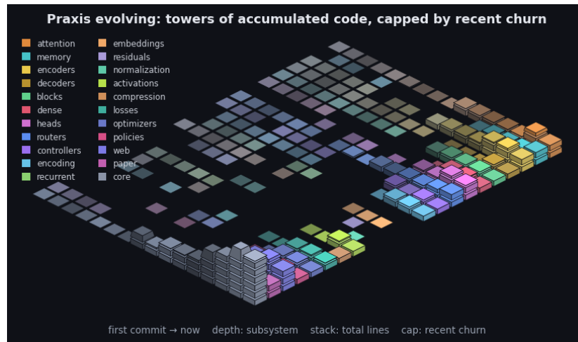
Figure 13: Praxis’s git history as an isometric terrain over the last 2602 commits. Each cell is one subsystem in one time window: a stack of base blocks for its accumulated size (total lines, recency-weighted) topped by a vivid cap for that window’s line churn - the standing codebase carrying the recent activity. Both are weighted by recency (the kernel the model applies to a sequence, turned on the repository): recent windows stack tall with bright caps while history thins toward the always-present prior - the low valley we roll into. Color fades from each subsystem’s hue toward a neutral prior into the past, banded in phased strata over a non-linear timescale. It is the bias/variance geometry read along the frequency axis (see the project notes): loud recent corrections over the quiet, ever-present base. By recency-weighted churn the current center of gravity is core, web, paper. The framework charts the hand that builds it.
