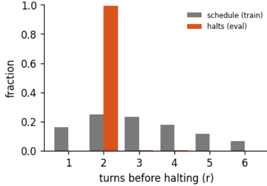
Figure 9: Halting distribution: the fraction of forward passes that stop after r turns, for the 6-turn recurrent loop of run abstractinator-u, early-halt rate 50%, mean boundary KL 0.661. schedule is the random loop-count the model trains under; halts is where the KL gate actually stops at inference. A mass pinned at the maximum (KL never collapsing) is the honest signature of a model that has not yet learned to converge early - the decision is real, not yet decisive.
