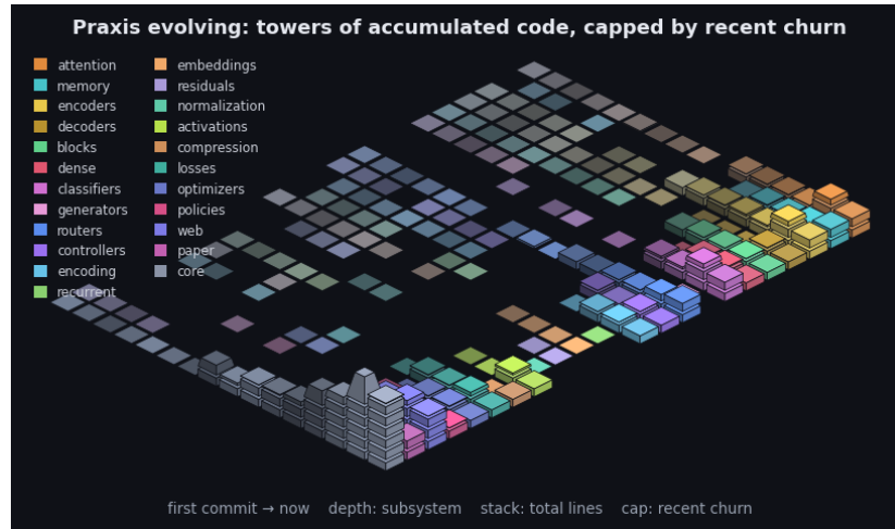
Figure 9: Praxis’s git history as an isometric terrain over the last 2623 commits. Each cell is one subsystem in one time window: a stack of base blocks for its accumulated size (total lines, recency-weighted) topped by a vivid cap for that window’s line churn - the standing codebase carrying the recent activity. Both are weighted by recency (the kernel the model applies to a sequence, turned on the repository): recent windows stack tall with bright caps while history thins toward the always-present prior - the low valley we roll into. Color fades from each subsystem’s hue toward a neutral prior into the past, banded in phased strata over a non-linear timescale. It is the bias/variance geometry read along the frequency axis (see the project notes): loud recent corrections over the quiet, ever-present base. By recency-weighted churn the current center of gravity is core, web, encoders. The framework charts the hand that builds it.
