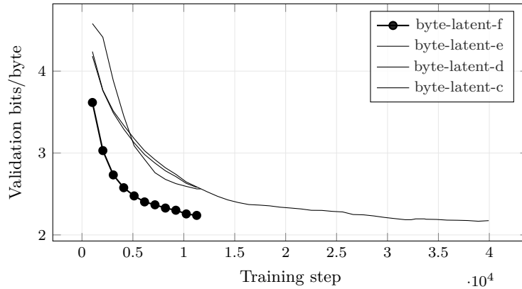
Figure 10: Bits per Byte across the 4 most recent experiments with comparable validation curves; the current experiment (byte-latent-f) is drawn in bold. Bold marks which run this build is reporting on , not which run scores best. The curves end wherever each run stopped, so they are at different points along their own training, and their endpoints are not a ranking. Generated from run logs - metrics that are not comparable across families (token loss vs. byte bits-per-byte vs. codec/CALM BrierLM) are excluded by construction, so the curves on this axis mean the same thing.
