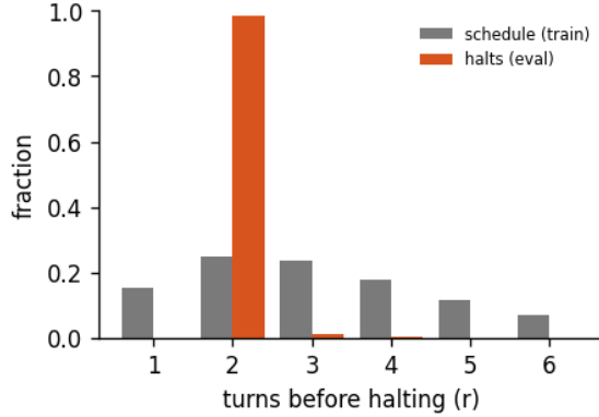
Figure 9: Halting distribution: the fraction of forward passes that stop after r turns, for the 6-turn recurrent loop of run abstractinator-c, early-halt rate 50%, mean boundary KL 1.34. schedule is the random loop-count the model trains under; halts is where the KL gate actually stops at inference. A mass pinned at the maximum (KL never collapsing) is the honest signature of a model that has not yet learned to converge early - the decision is real, not yet decisive.
