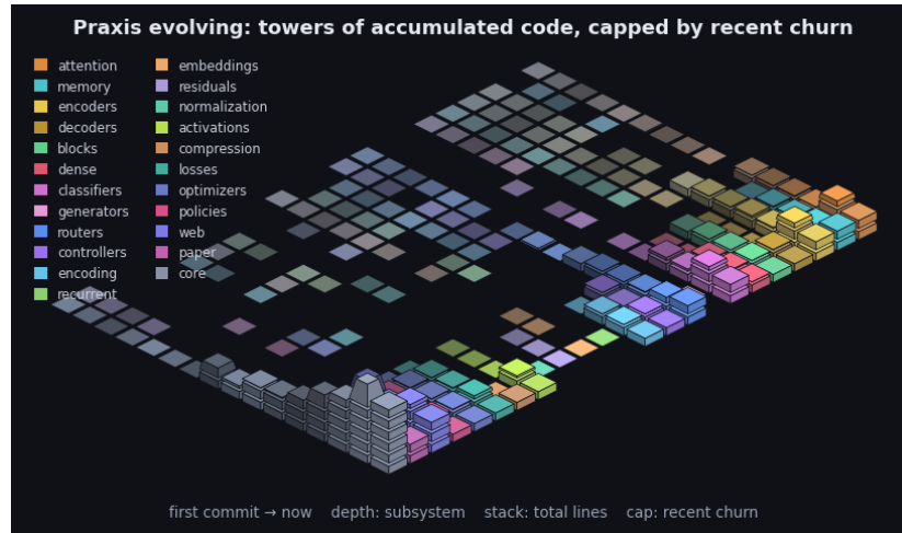
Figure 9: Praxis’s git history as an isometric terrain over the last 2664 commits. Each cell is one subsystem in one time window: a stack of base blocks for its accumulated size (total lines, recency-weighted) topped by a vivid cap for that window’s line churn - the standing codebase carrying the recent activity. Both are weighted by recency (the kernel the model applies to a sequence, turned on the repository): recent windows stack tall with bright caps while history thins toward the always-present prior - the low valley we roll into. Color fades from each subsystem’s hue toward a neutral prior into the past, banded in phased strata over a non-linear timescale. It is the bias/variance geometry read along the frequency axis (see the project notes): loud recent corrections over the quiet, ever-present base. By recency-weighted churn the current center of gravity is core, web, encoders. The framework charts the hand that builds it.
