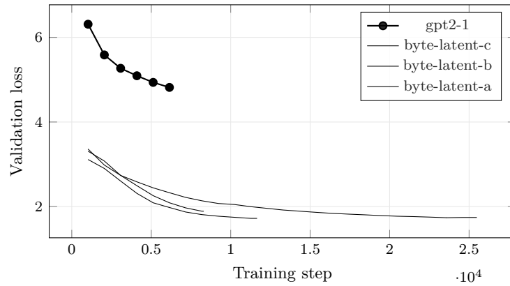
Figure 10: Validation Loss across the 4 most recent experiments with comparable validation curves; the current experiment (gpt2-1) is drawn in bold. Bold marks which run this build is reporting on , not which run scores best. The curves end wherever each run stopped, so they are at different points along their own training, and their endpoints are not a ranking. Generated from run logs - metrics that are not comparable across families (token loss vs. byte bits-per-byte vs. codec/CALM BrierLM) are excluded by construction, so the curves on this axis mean the same thing.
