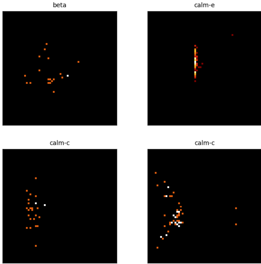
Figure 2: Center PCA density for the 4 most recent crystal-head runs (beta, calm-e, calm-c, calm-c). Each panel is the top-2 PCA projection of a head's vocabulary centers, binned to a 64 \times 64 density grid (log color) - the same snapshot the dashboard renders live. Different runs settle into structurally different geometries, not noise.
