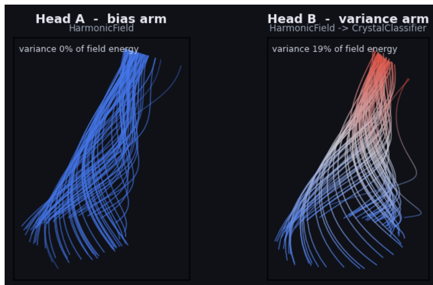
Figure 4: The prismatic head's two arms, rendered exactly as the dashboard's bias/variance strand card. Each hair is one feature, morphing from a ring (its static-field phase) out to its (bias, variance) position with a helical twist; color runs blue (pure bias) to red (pure variance). Head A (left) is the bias arm: it reads a static field, so every hair stays blue - a constant structural vote. Head B (right) is the variance arm, whose input-conditional envelope lets hairs swing toward red - the data-dependent vote. Each panel's subtitle lists that arm's head stack. The two together are the orthogonal bias/variance decomposition made architectural - convex and radial from the center, chaotic in the arms.
