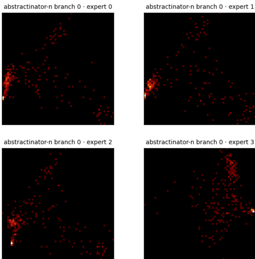
Figure 11: Center PCA density for the 4 crystal heads of abstractinator-n - a single multi-head model (prismatic6’s VEAR crystal bank), so these are that run’s own heads (branch 0 · expert 0, branch 0 · expert 1, branch 0 · expert 2, branch 0 · expert 3), not a cross-run mix. Each panel is the top-2 PCA projection of a head’s vocabulary centers, binned to a 64 \times 64 density grid (log color) - the same snapshot the dashboard renders live. The bank’s experts settle into structurally distinct geometries - the between-expert variance the router selects over.
