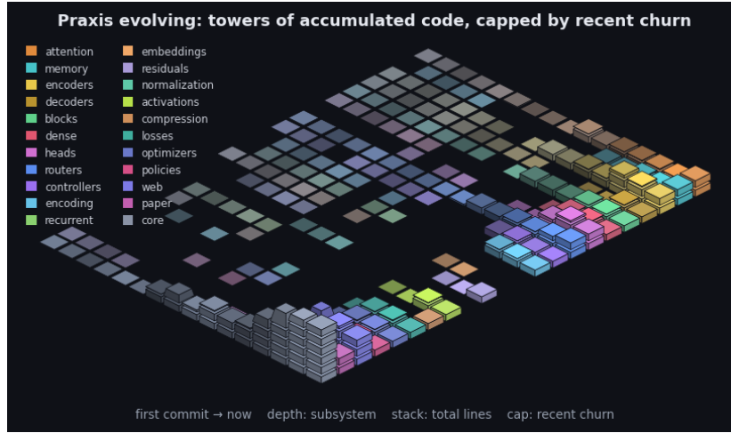
Figure 12: Praxis’s git history as an isometric terrain over the last 2516 commits. Each cell is one subsystem in one time window: a stack of base blocks for its accumulated size (total lines, recency-weighted) topped by a vivid cap for that window’s line churn - the standing codebase carrying the recent activity. Both are weighted by recency (the kernel the model applies to a sequence, turned on the repository): recent windows stack tall with bright caps while history thins toward the always-present prior - the low valley we roll into. Color fades from each subsystem’s hue toward a neutral prior into the past, banded in phased strata over a non-linear timescale. It is the bias/variance geometry read along the frequency axis (see the project notes): loud recent corrections over the quiet, ever-present base. By recency-weighted churn the current center of gravity is core, web, paper. The framework charts the hand that builds it.
