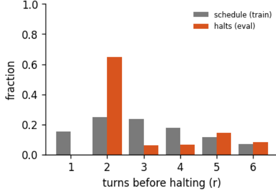
Figure 8: Halting distribution: the fraction of forward passes that stop after r turns, for the 6-turn recurrent loop of run abstractinator-n, early-halt rate 32%, mean boundary KL 0.522. schedule is the random loop-count the model trains under; halts is where the KL gate actually stops at inference. A mass pinned at the maximum (KL never collapsing) is the honest signature of a model that has not yet learned to converge early - the decision is real, not yet decisive.
