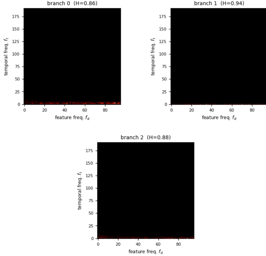
Figure 2: The static amplitude spectrum |a[f_t, f_d]| across the 3 arms of abstractinator-a’s prismatic head - the learned grid that, inverse-transformed through the frozen Weyl phases, becomes the bias field. This is the heatmap the text describes: energy that settles into a low-frequency band (small f_t, f_d ) is the corpus rhythm crystallizing, while a grid that stays uniform is a field still indistinguishable from noise. Hoyer concentrations H = 0.86, 0.94, 0.88 (left to right) quantifies it on the same [0, 1] scale the prose names (1 = a single cell, 0 = uniform), computed from this very tensor by concentration() - the same value the dashboard logs live. The pink 1/f^\alpha prior lives in the frozen basis, not in these amplitudes, so the grid shown is exactly what the head exposes.
