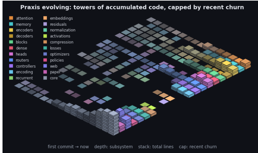
Figure 10: Praxis’s git history as an isometric terrain over the last 2407 commits. Each cell is one subsystem in one time window: a stack of base blocks for its accumulated size (total lines, recency-weighted) topped by a vivid cap for that window’s line churn - the standing codebase carrying the recent activity. Both are weighted by recency (the kernel the model applies to a sequence, turned on the repository): recent windows stack tall with bright caps while history thins toward the always-present prior - the low valley we roll into. Color fades from each subsystem’s hue toward a neutral prior into the past, banded in phased strata over a non-linear timescale. It is the bias/variance geometry read along the frequency axis (see the project notes): loud recent corrections over the quiet, ever-present base. By recency-weighted churn the current center of gravity is core, web, paper. The framework charts the hand that builds it.
