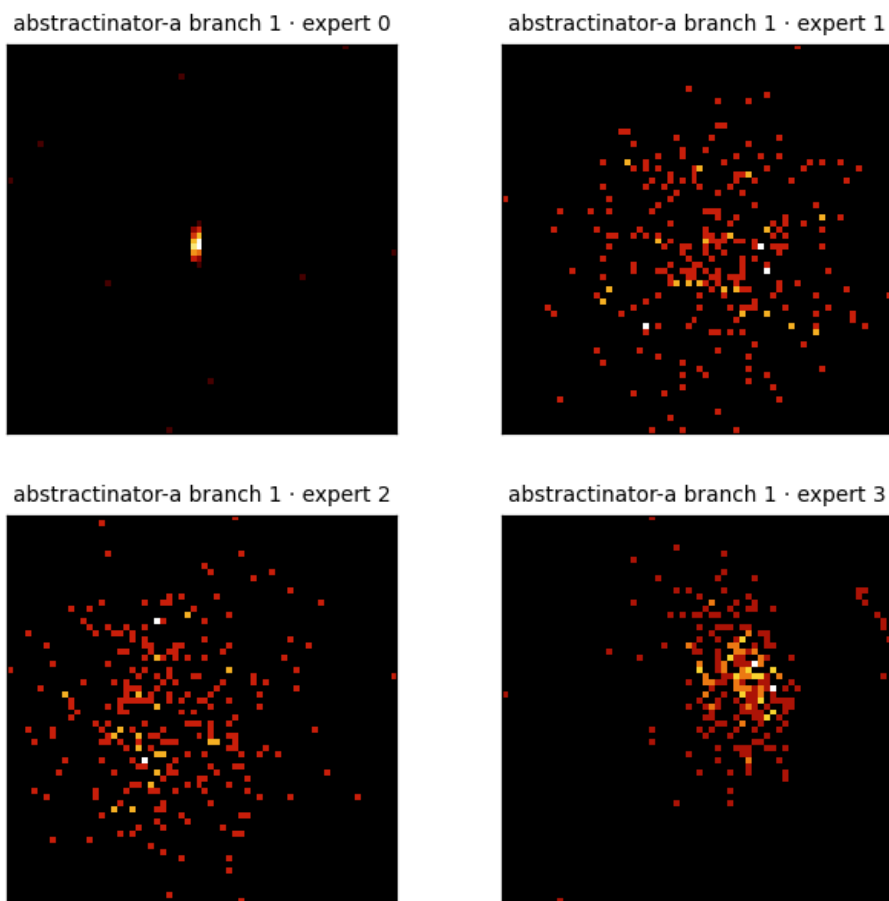
Figure 9: Center PCA density for the 4 crystal heads of abstractinator-a - a single multi-head model (prismatic4’s VEAR crystal bank), so these are that run’s own heads (branch 1 · expert 0, branch 1 · expert 1, branch 1 · expert 2, branch 1 · expert 3), not a cross-run mix. Each panel is the top-2 PCA projection of a head’s vocabulary centers, binned to a 64 \times 64 density grid (log color) - the same snapshot the dashboard renders live. The bank’s experts settle into structurally distinct geometries - the between-expert variance the router selects over.
