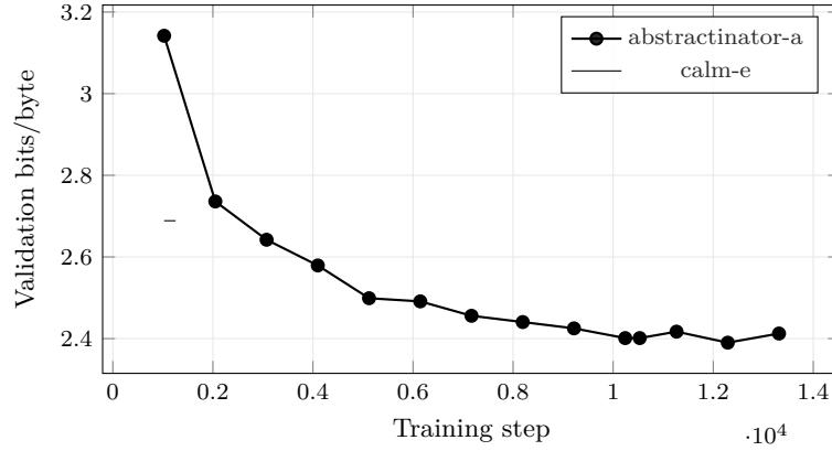
Figure 11: Bits per Byte across the 2 most recent experiments with comparable validation curves; the leading run (abstractinator-a) is drawn in bold. Generated from run logs - metrics that are not comparable across families (token loss vs. byte bits-per-byte vs. codec/CALM BrierLM) are excluded by construction, so the curves on this axis mean the same thing.
