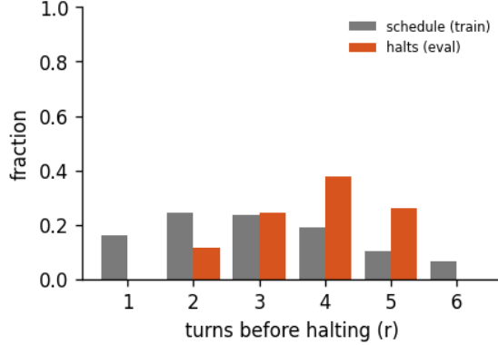
Figure 9: Halting distribution: the fraction of forward passes that stop after r turns, for the 6-turn recurrent loop of run abstractinator-x, early-halt rate 26%, mean boundary KL 0.309. schedule is the random loop-count the model trains under; halts is where the KL gate actually stops at inference. A mass pinned at the maximum (KL never collapsing) is the honest signature of a model that has not yet learned to converge early - the decision is real, not yet decisive.
