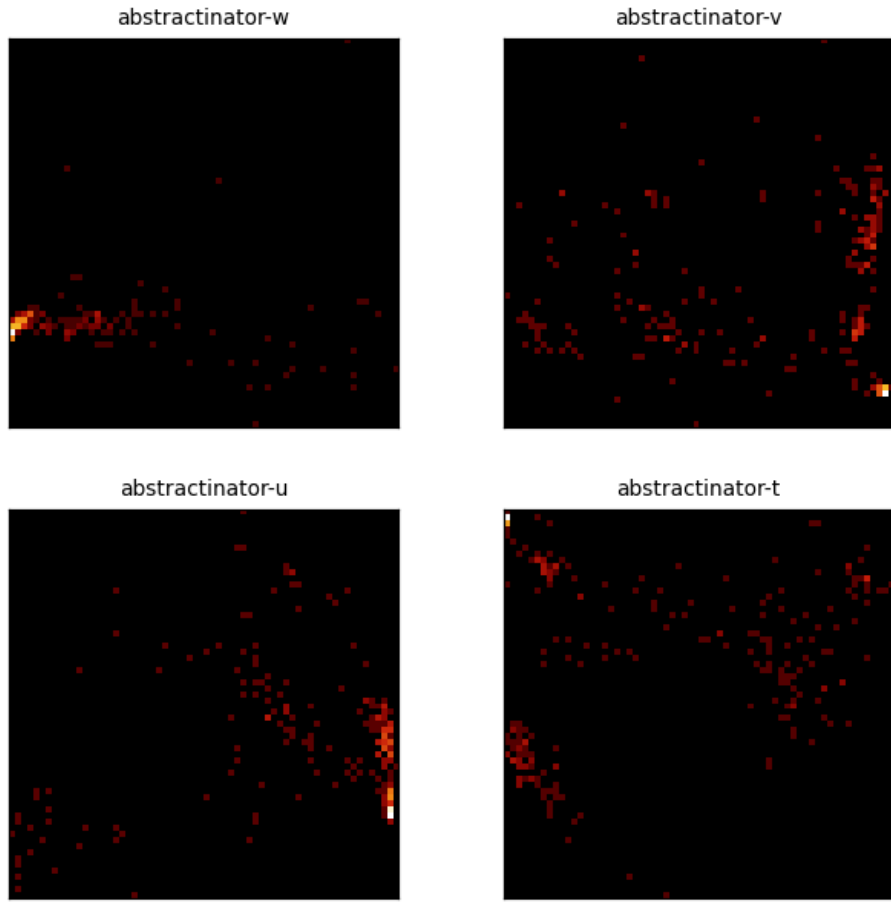
Figure 12: Center PCA density for the 4 most recent crystal-head runs (abstractinator-w, abstractinator-v, abstractinator-u, abstractinator-t). Each panel is the top-2 PCA projection of a head’s vocabulary centers, binned to a 64 \times 64 density grid (log color) - the same snapshot the dashboard renders live. Different runs settle into structurally different geometries, not noise.
