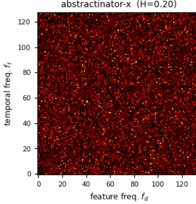
Figure 2: The static amplitude spectrum |a[f_t, f_d]| for abstractinator-x - the learned grid that, inverse-transformed through the frozen Weyl phases, becomes the bias field. This is the heatmap the text describes: energy that settles into a low-frequency band (small f_t, f_d ) is the corpus rhythm crystallizing, while a grid that stays uniform is a field still indistinguishable from noise. Hoyer concentration H = 0.20 quantifies it on the same [0, 1] scale the prose names (1 = a single cell, 0 = uniform), computed from this very tensor - the same value the dashboard logs live. The pink 1/f^\alpha prior lives in the frozen basis, not in these amplitudes, so the grid shown is exactly what the head exposes.
