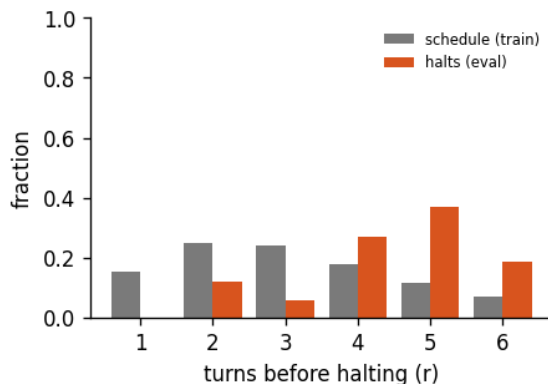
Figure 8: Halting distribution: the fraction of forward passes that stop after r turns, for the 6-turn recurrent loop of run abstractinator-s, early-halt rate 19%, mean boundary KL 0.378. schedule is the random loop-count the model trains under; halts is where the KL gate actually stops at inference. A mass pinned at the maximum (KL never collapsing) is the honest signature of a model that has not yet learned to converge early - the decision is real, not yet decisive.
