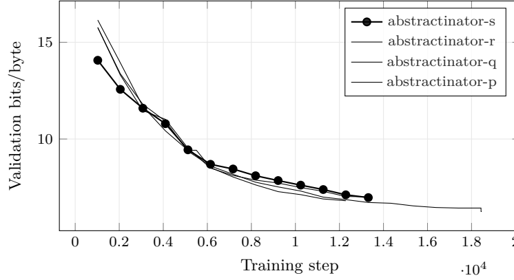
Figure 13: Bits per Byte across the 4 most recent experiments with comparable validation curves; the current experiment (abstractinator-s) is drawn in bold. Bold marks which run this build is reporting on , not which run scores best. The curves end wherever each run stopped, so they are at different points along their own training, and their endpoints are not a ranking. Generated from run logs - metrics that are not comparable across families (token loss vs. byte bits-per-byte vs. codec/CALM BrierLM) are excluded by construction, so the curves on this axis mean the same thing.
