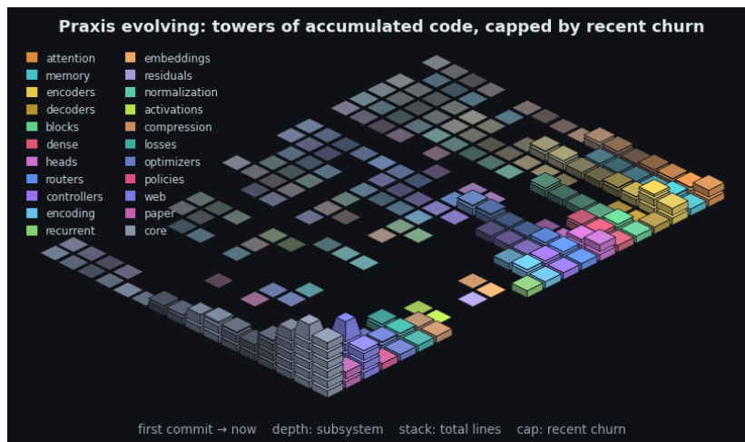
Figure 4: Praxis’s git history as an isometric terrain over the last 2302 commits. Each cell is one subsystem in one time window: a stack of base blocks for its accumulated size (total lines, recency-weighted) topped by a vivid cap for that window’s line churn - the standing codebase carrying the recent activity. Both are weighted by recency (the kernel the model applies to a sequence, turned on the repository): recent windows stack tall with bright caps while history thins toward the always-present prior - the low valley we roll into. Color fades from each subsystem’s hue toward a neutral prior into the past, banded in phased strata over a non-linear timescale. It is the bias/variance geometry read along the frequency axis (see the project notes): loud recent corrections over the quiet, ever-present base. By recency-weighted churn the current center of gravity is core, web, paper. The framework charts the hand that builds it.
