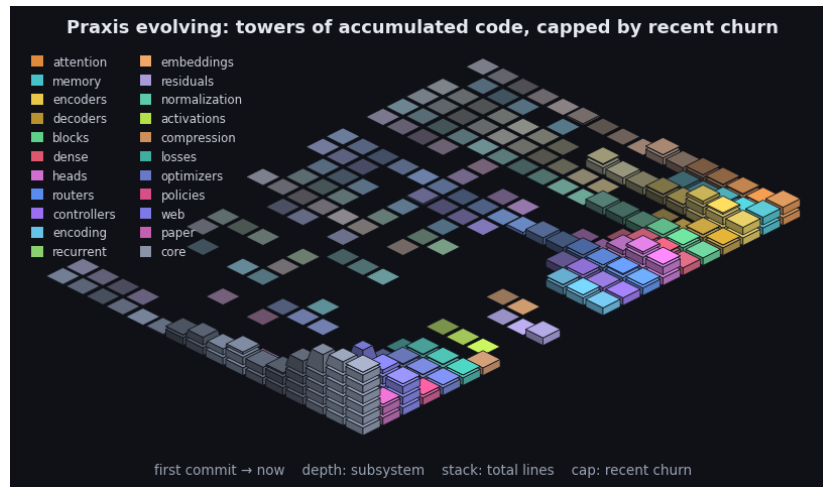
Figure 12: Praxis's git history as an isometric terrain over the last 2478 commits. Each cell is one subsystem in one time window: a stack of base blocks for its accumulated size (total lines, recency-weighted) topped by a vivid cap for that window's line churn - the standing codebase carrying the recent activity. Both are weighted by recency (the kernel the model applies to a sequence, turned on the repository): recent windows stack tall with bright caps while history thins toward the always-present prior - the low valley we roll into. Color fades from each subsystem's hue toward a neutral prior into the past, banded in phased strata over a non-linear timescale. It is the bias/variance geometry read along the frequency axis (see the project notes): loud recent corrections over the quiet, ever-present base. By recency-weighted churn the current center of gravity is core, web, paper. The framework charts the hand that builds it.
