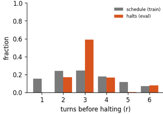
Figure 8: Halting distribution: the fraction of forward passes that stop after r turns, for the 6-turn recurrent loop of run abstractinator-h, early-halt rate 29%, mean boundary KL 0.227. schedule is the random loop-count the model trains under; halts is where the KL gate actually stops at inference. A mass pinned at the maximum (KL never collapsing) is the honest signature of a model that has not yet learned to converge early - the decision is real, not yet decisive.
