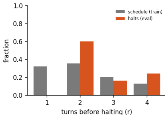
Figure 8: Halting distribution: the fraction of forward passes that stop after r turns, for the 4-turn recurrent loop of run abstractinator-g, early-halt rate 32%, mean boundary KL 0.474. schedule is the random loop-count the model trains under; halts is where the KL gate actually stops at inference. A mass pinned at the maximum (KL never collapsing) is the honest signature of a model that has not yet learned to converge early - the decision is real, not yet decisive.
