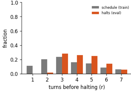
Figure 6: Halting distribution: the fraction of forward passes that stop after r turns, for the 7-turn recurrent loop of run abstractinator-b, early-halt rate 22%, mean boundary KL 0.194. schedule is the random loop-count the model trains under; halts is where the KL gate actually stops at inference. A mass pinned at the maximum (KL never collapsing) is the honest signature of a model that has not yet learned to converge early - the decision is real, not yet decisive.
