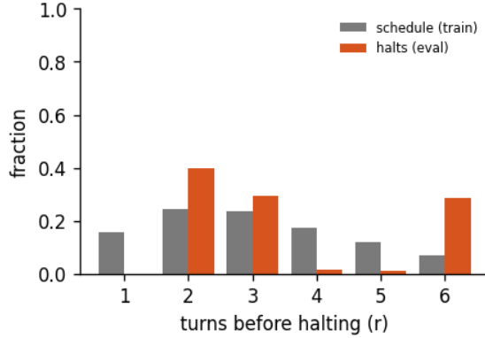
Figure 8: Halting distribution: the fraction of forward passes that stop after r turns, for the 6-turn recurrent loop of run abstractinator-j, early-halt rate 22%, mean boundary KL 0.204. schedule is the random loop-count the model trains under; halts is where the KL gate actually stops at inference. A mass pinned at the maximum (KL never collapsing) is the honest signature of a model that has not yet learned to converge early - the decision is real, not yet decisive.
